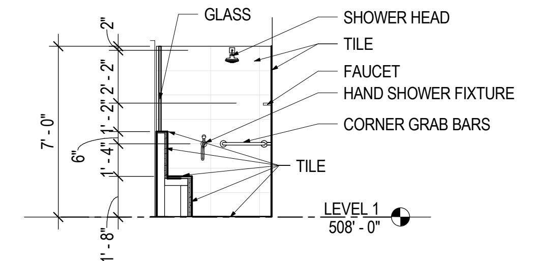
6 A7.02 MASTER BATHROOM 07 - SHOWER EAST 1/4" = 1'-0"
