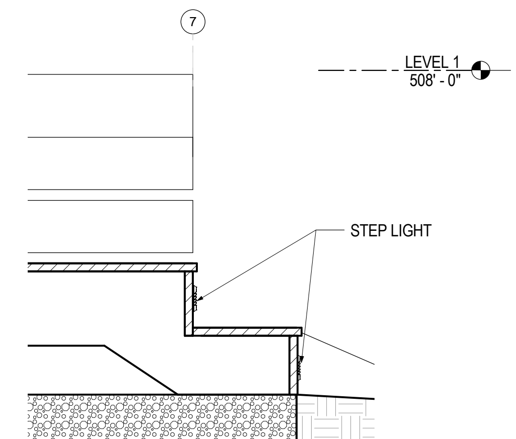
2 SECTION, SOUTH STAIR 1" = 1'-0"
