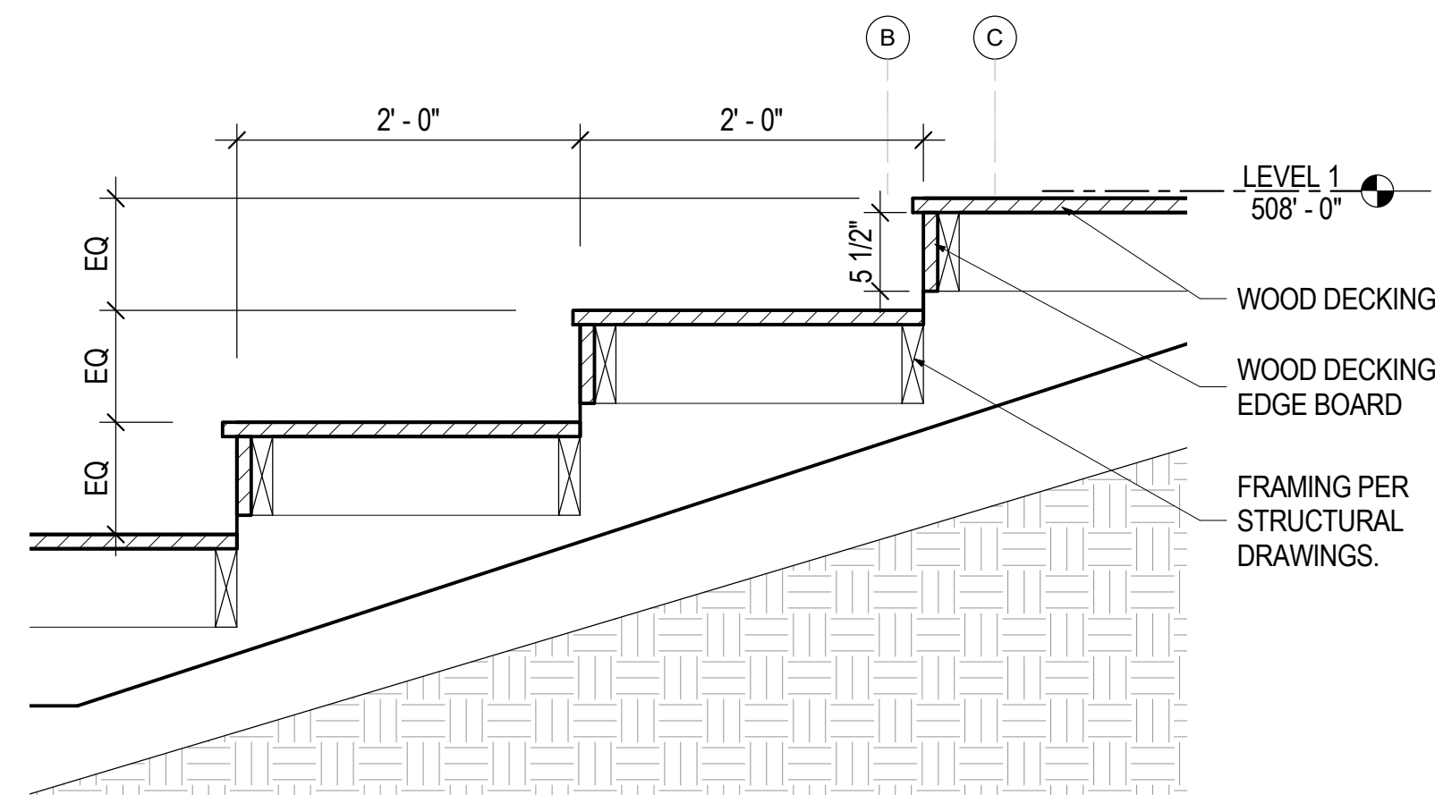
4 SECTION, WOOD STAIR 1" = 1'-0"
