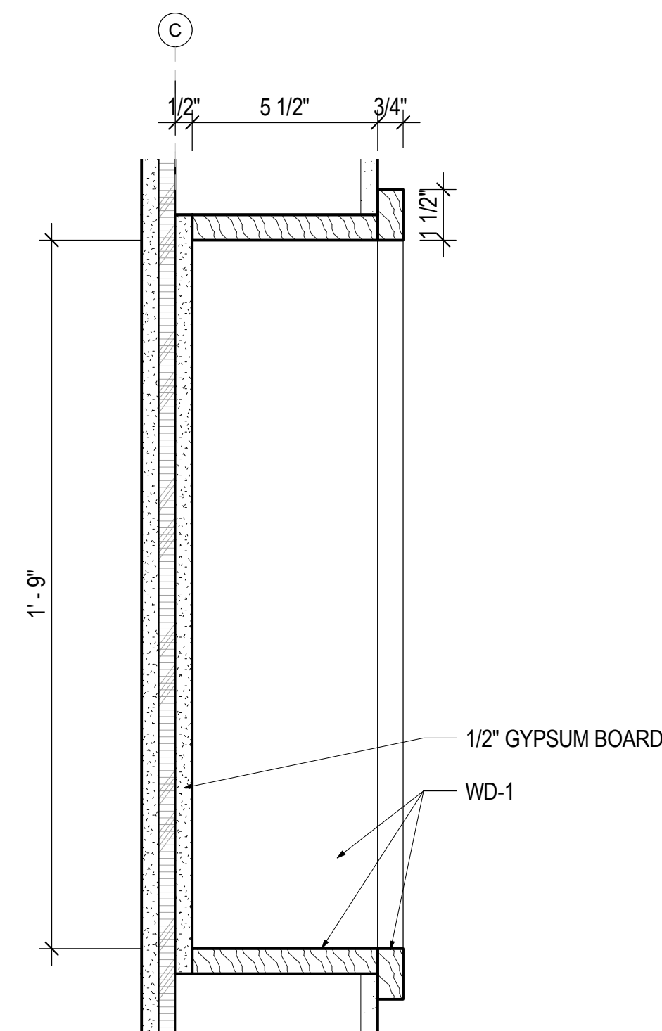
2 A7.10 SECTION, W-2 WALL SHELF, INTERIOR 3" = 1'-0"
