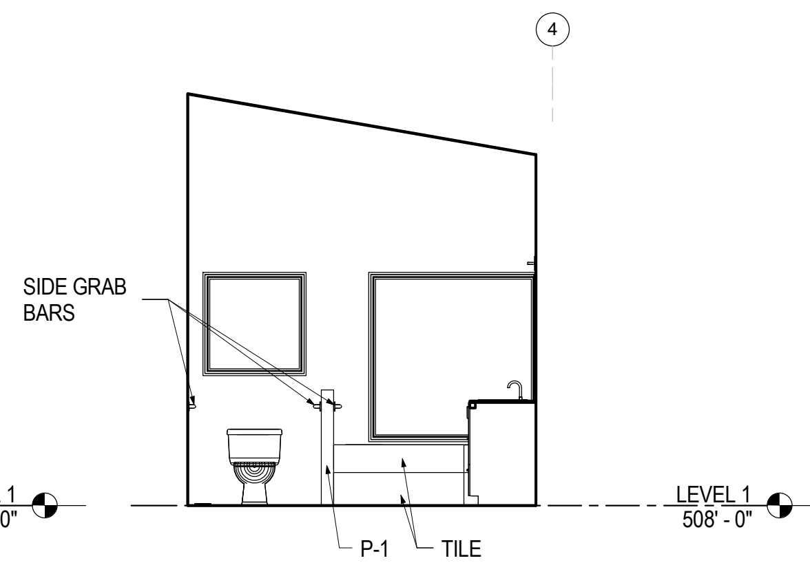
9 A7.02 MASTER BATHROOM 07 - WEST 1/4" = 1'-0"
