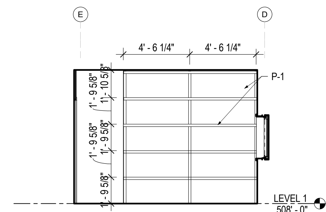
12 A7.02 LAUNDRY ROOM 12 - SOUTH 1/4" = 1'-0"
