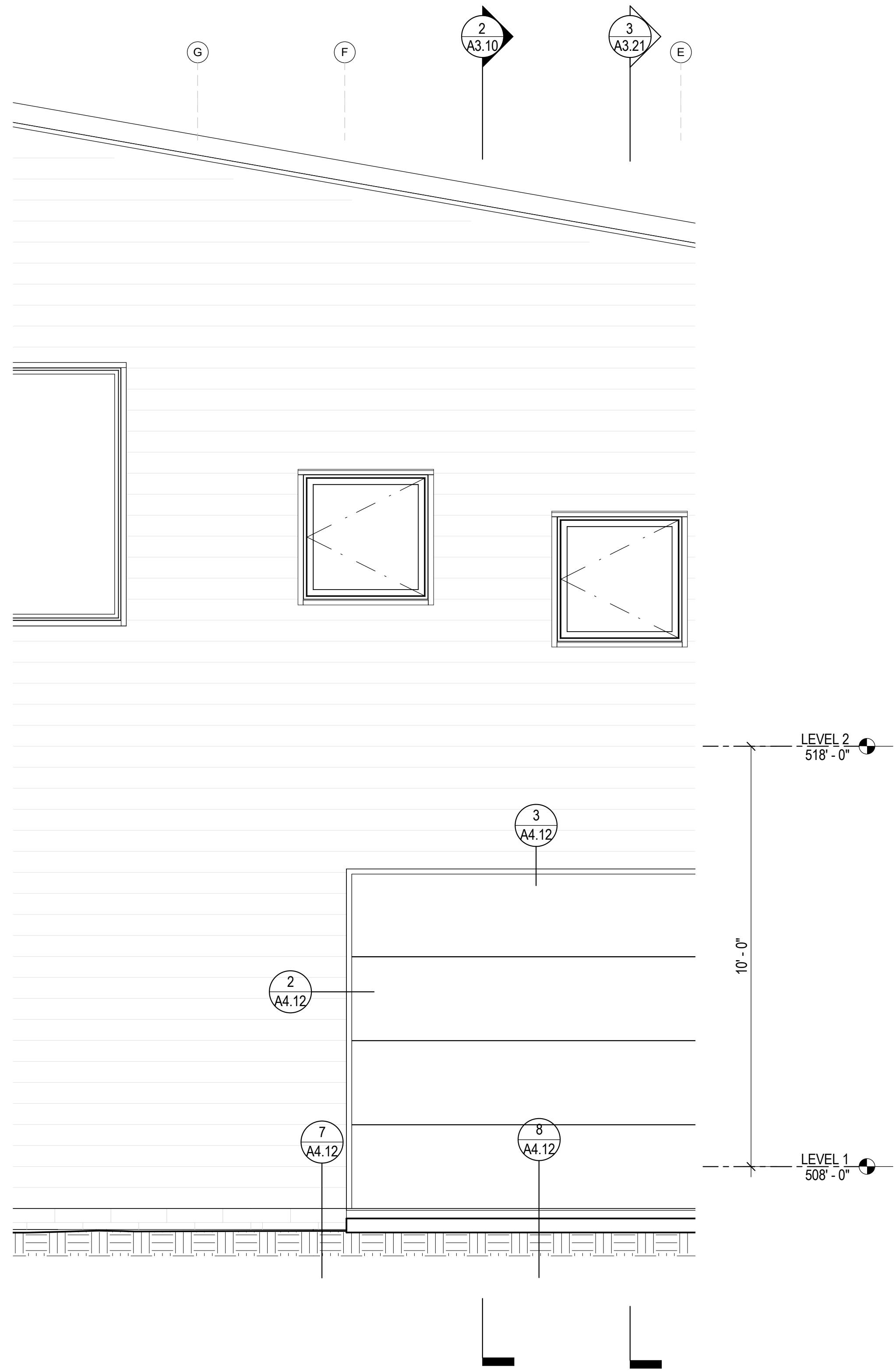
4 PARTIAL ELEVATION, GARAGE A3.21 1/2" = 1'-0"
