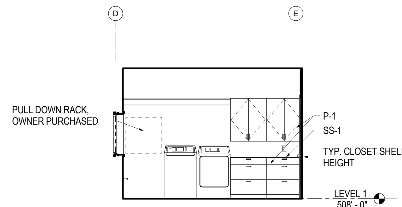
13 A7.02 LAUNDRY ROOM 12 - NORTH 1/4" = 1'-0"
