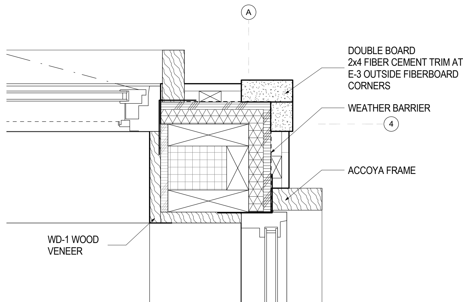
4 JAMB, BATHROOM WINDOW A4.13 3" = 1'-0"
