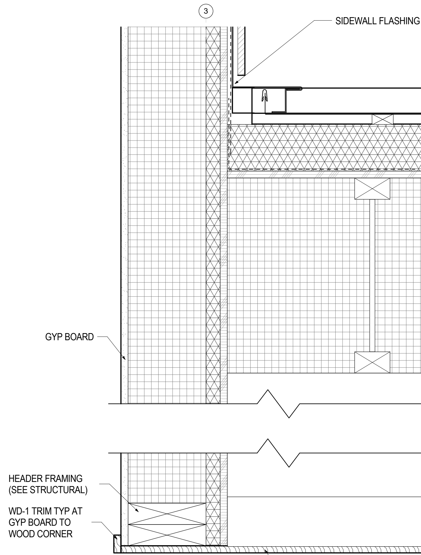
4 SECTION, ENTRY HALL ROOF A4.12 3" = 1'-0"
