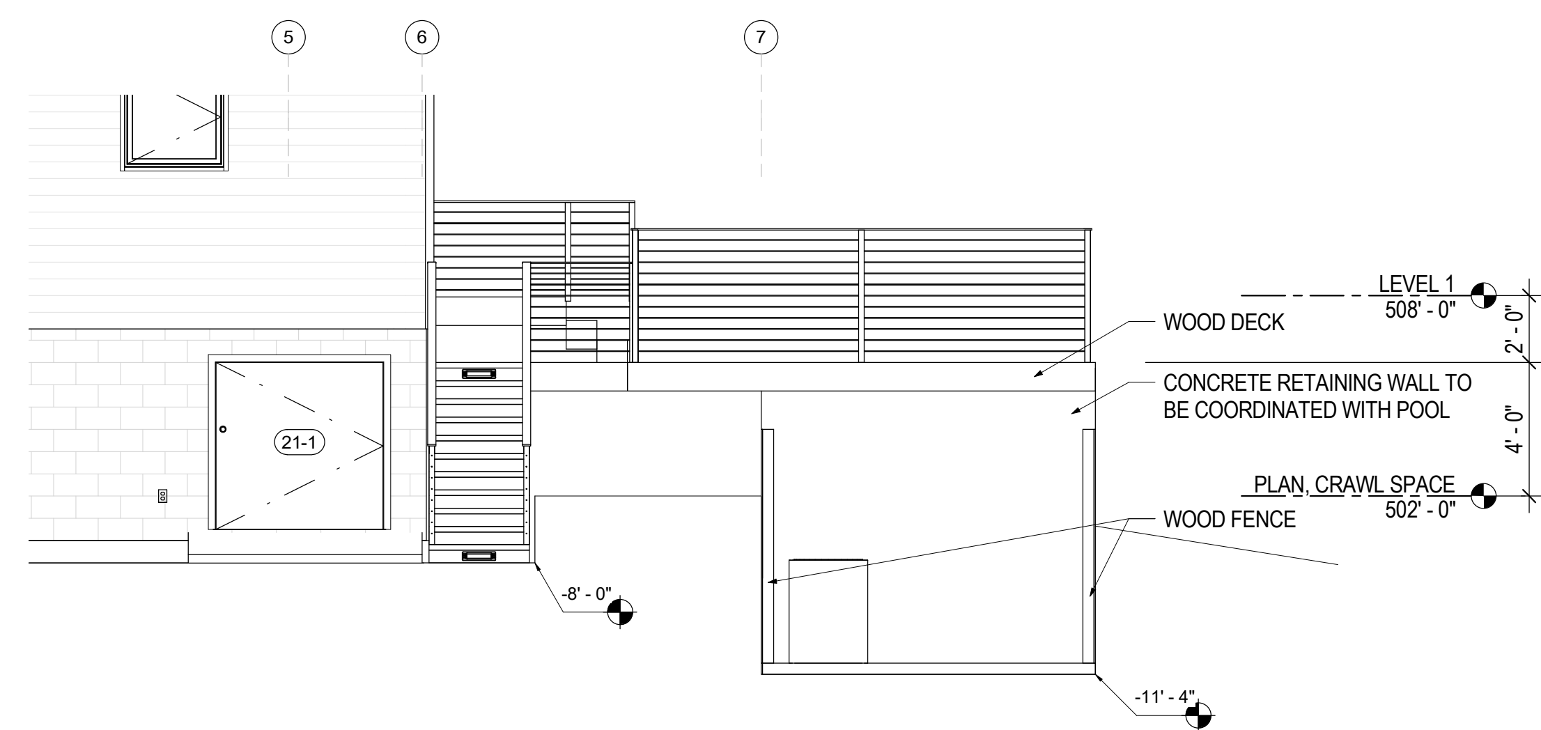
1 WEST ELEVATION, DECK A5.10 1/4" = 1'-0"
