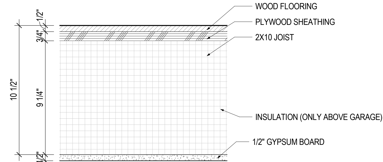
F-1 FLOOR ASSEMBLY, TYPICAL 3" = 1'-0"
