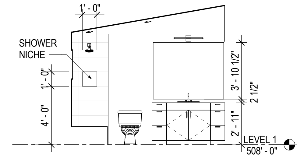
2 A7.02 BATHROOM 11 - EAST 1/4" = 1'-0"
