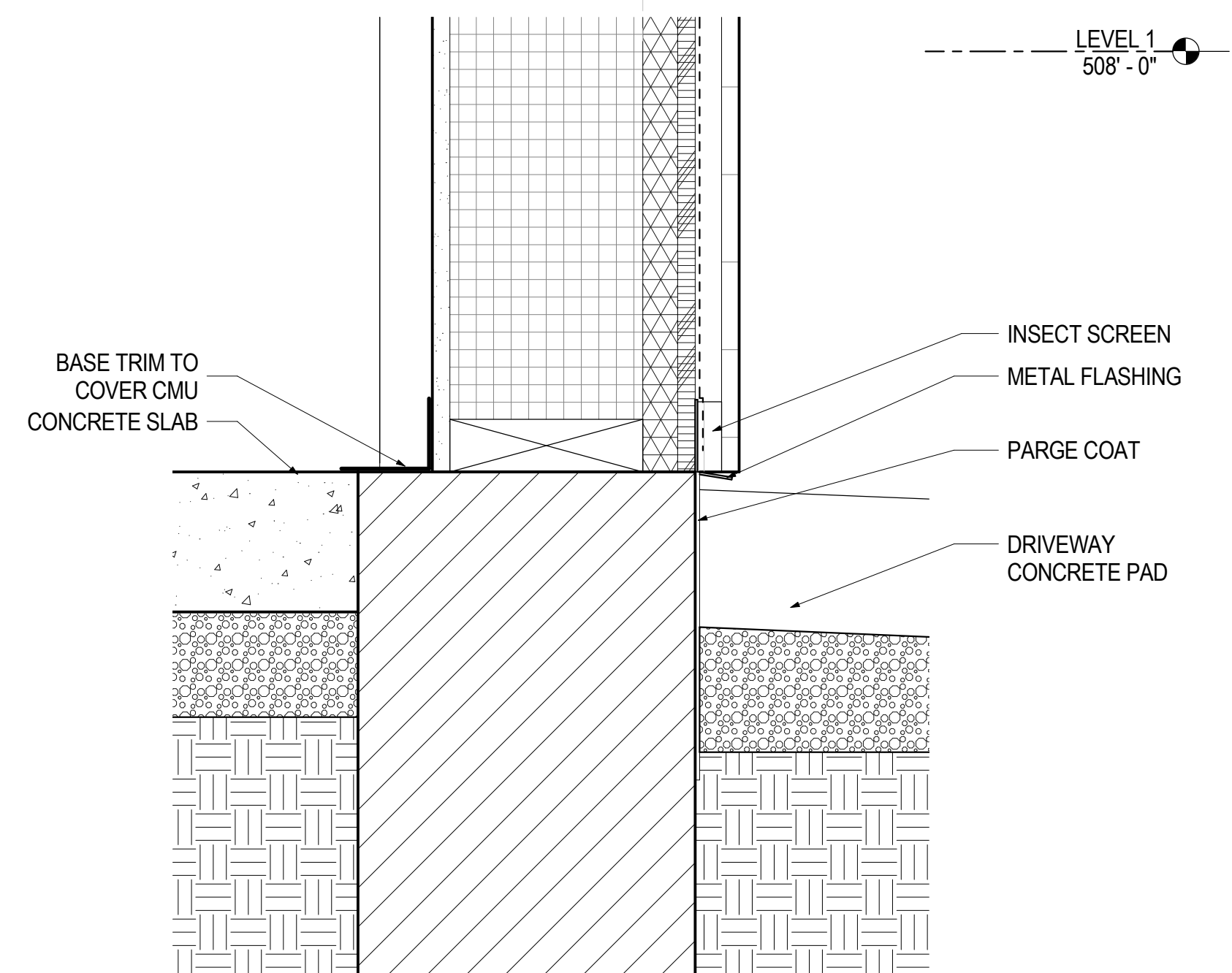
7 BASE, GARAGE A4.12 3" = 1'-0"
