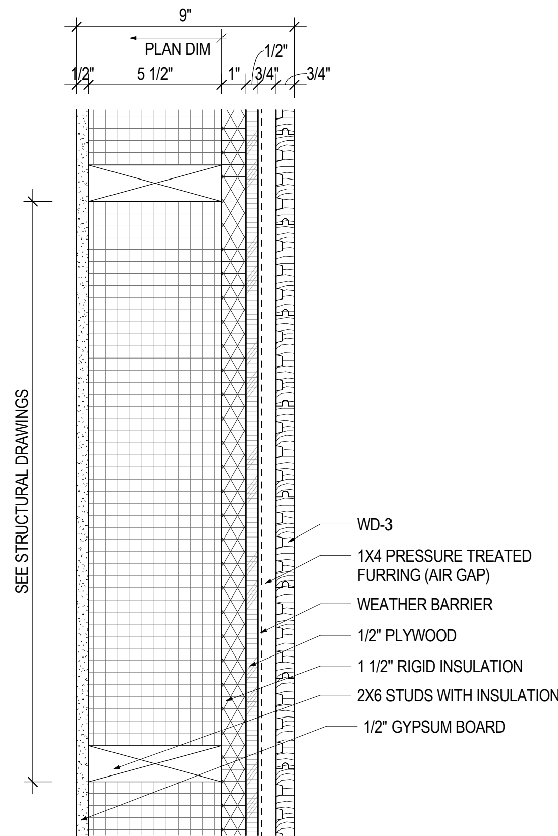
E-4 EXTERIOR WALL, WOOD 3" = 1'-0"
