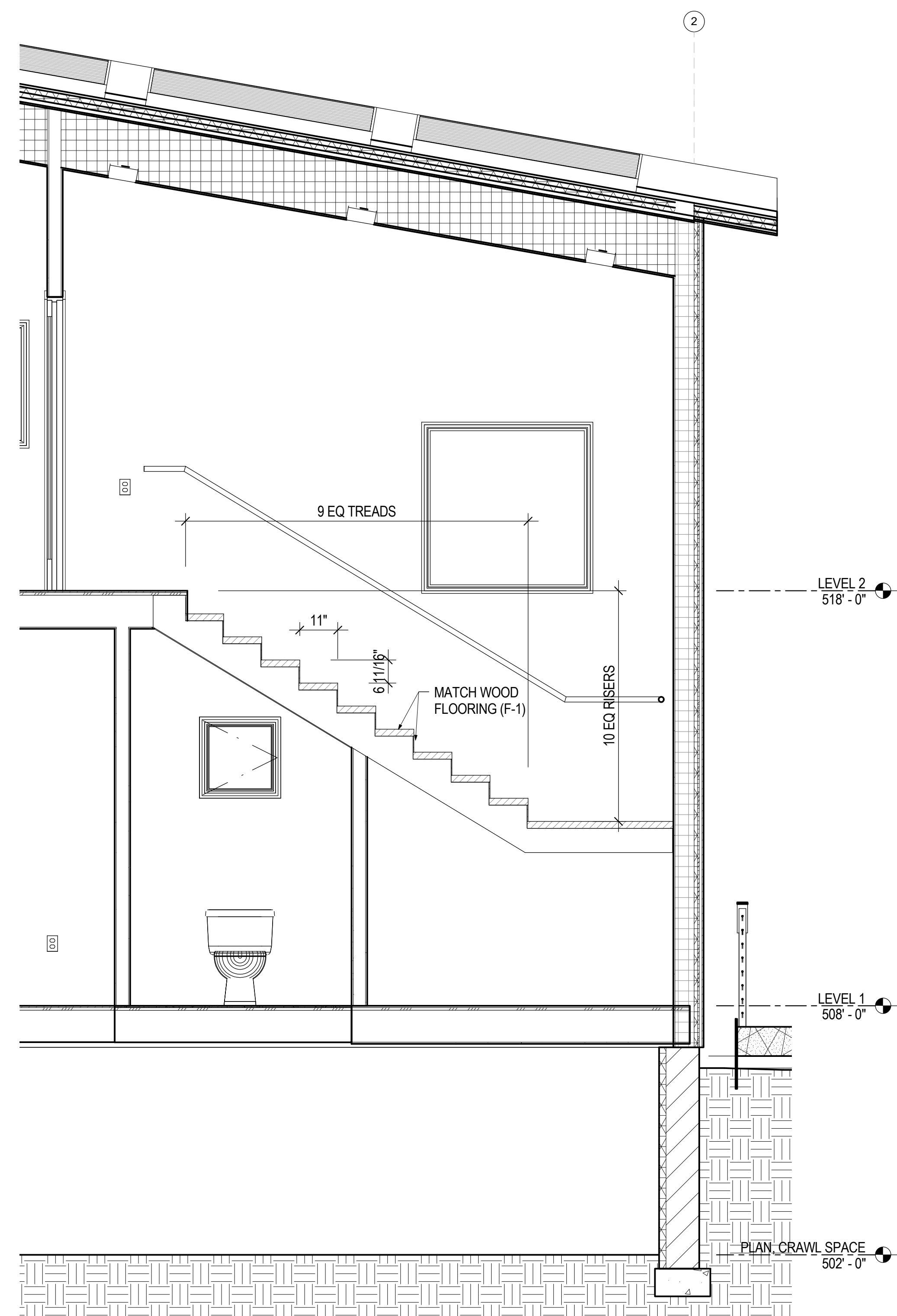
1 A3.22 SECTION, STAIRS EAST 1/2" = 1'-0"
