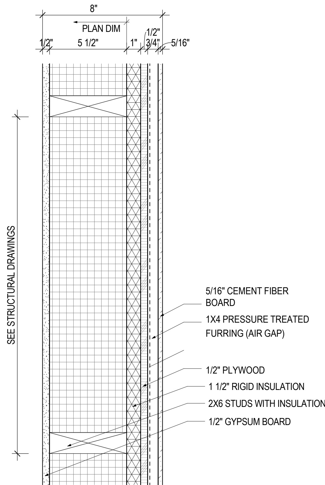
E-3 EXTERIOR WALL, FIBERBOARD 3" = 1'-0"
