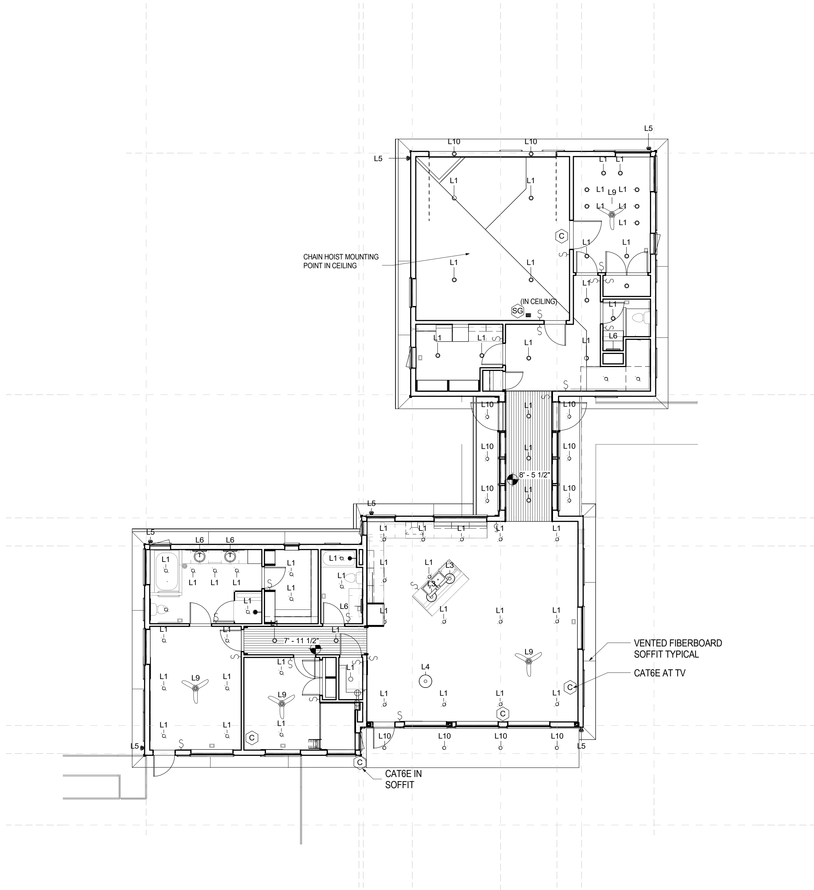
1 A6.01 REFLECTED CEILING PLAN, FIRST FLOOR 1/8" = 1'-0"
