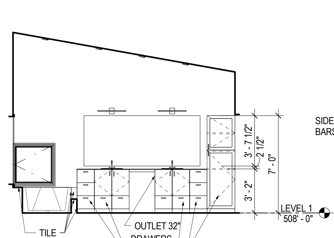
10 A7.02 MASTER BATHROOM 07 - NORTH 1/4" = 1'-0"
