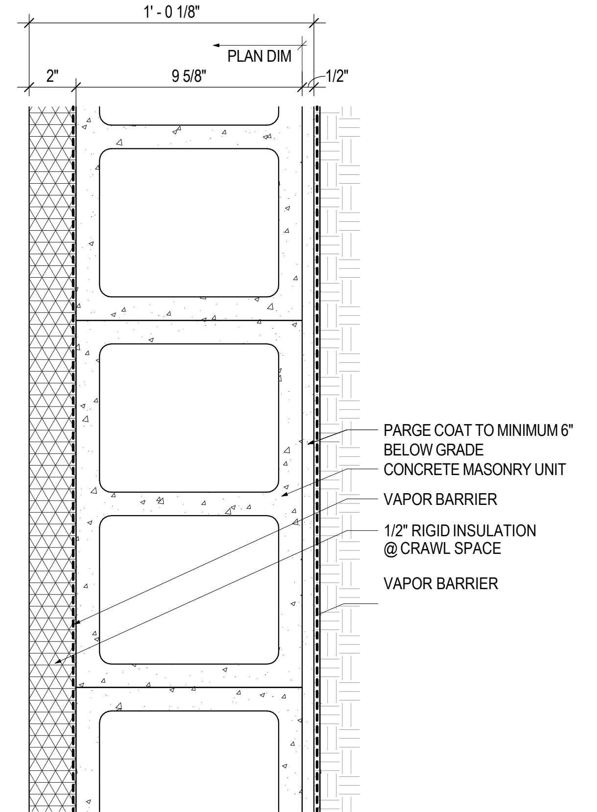
E-1 EXTERIOR WALL, CMU 3" = 1'-0"
