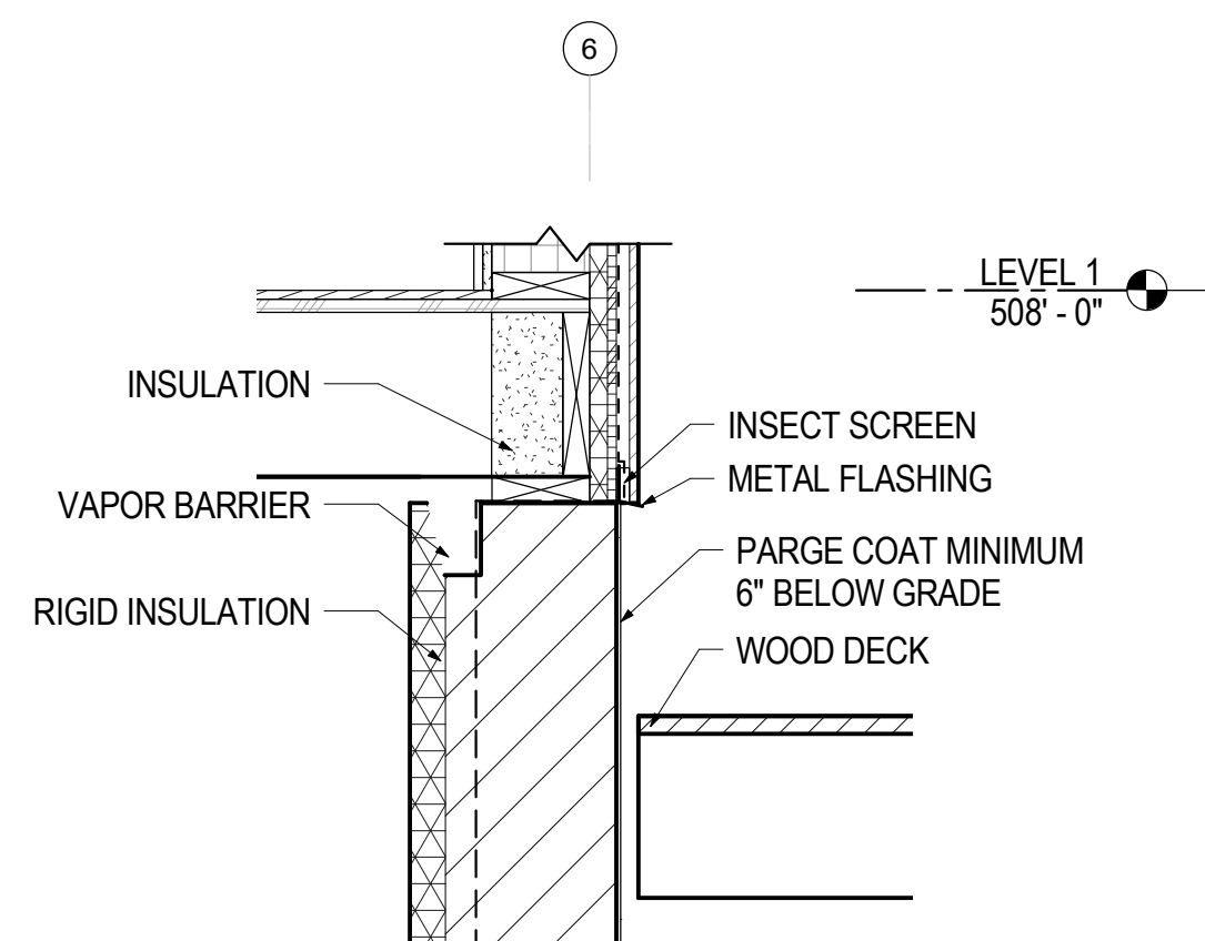
5 BASE, LOWER DECK 1" = 1'-0"
