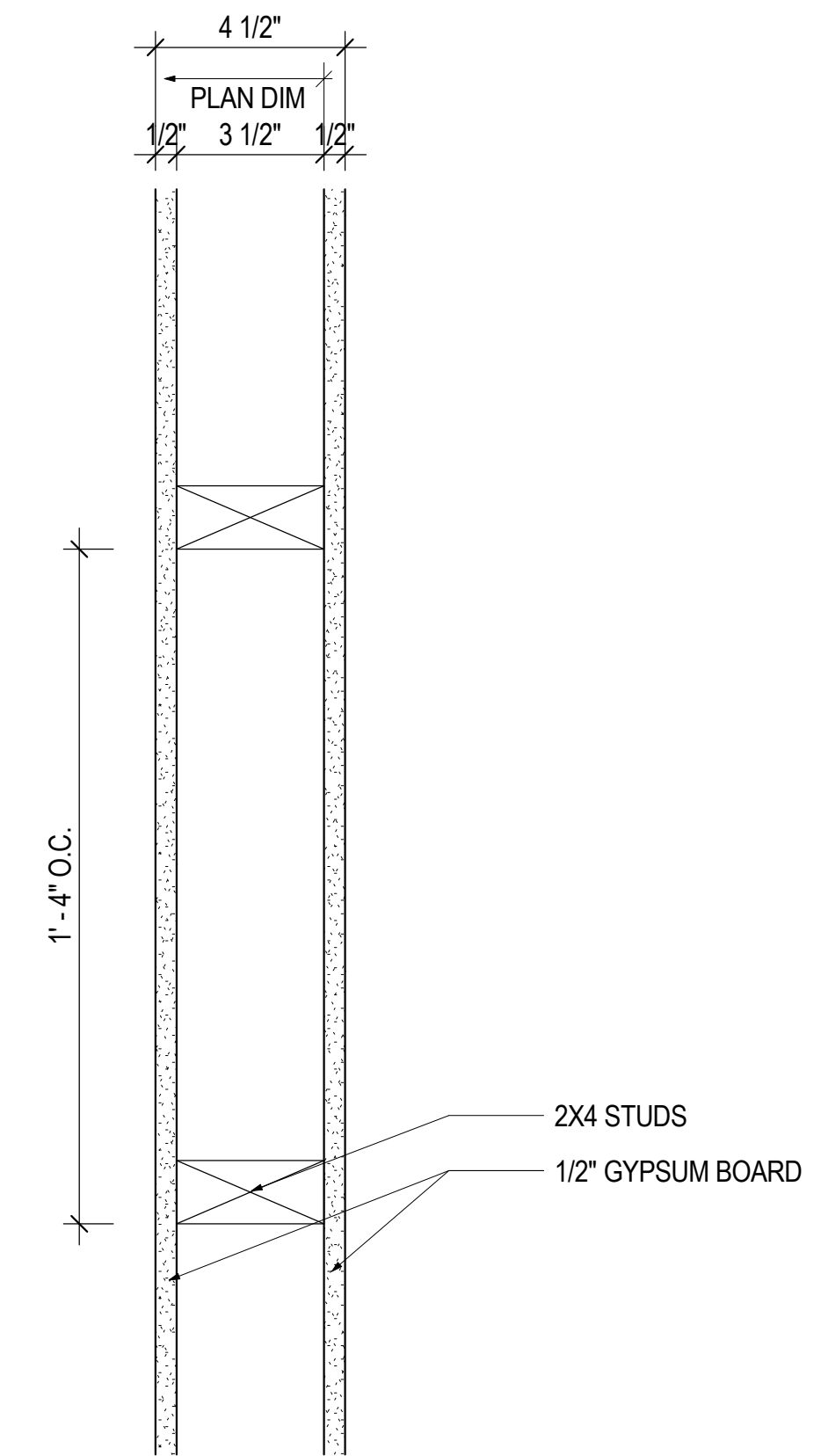
W-1 INTERIOR WALL, TYP 3" = 1'-0"
