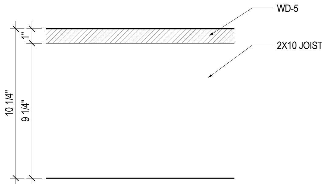
F-7 FLOOR ASSEMBLY, WOOD DECKING 3" = 1'-0"
