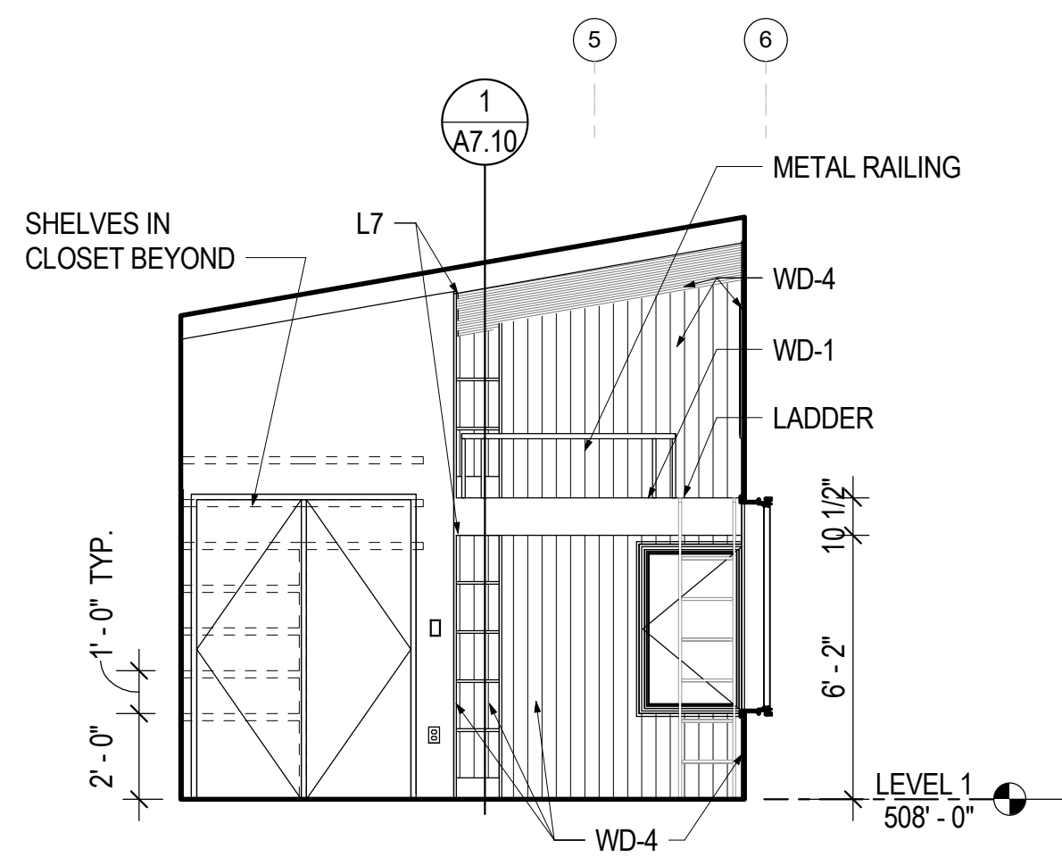
9 SECOND BEDROOM 09 - EAST A7.01 1/4" = 1'-0"
