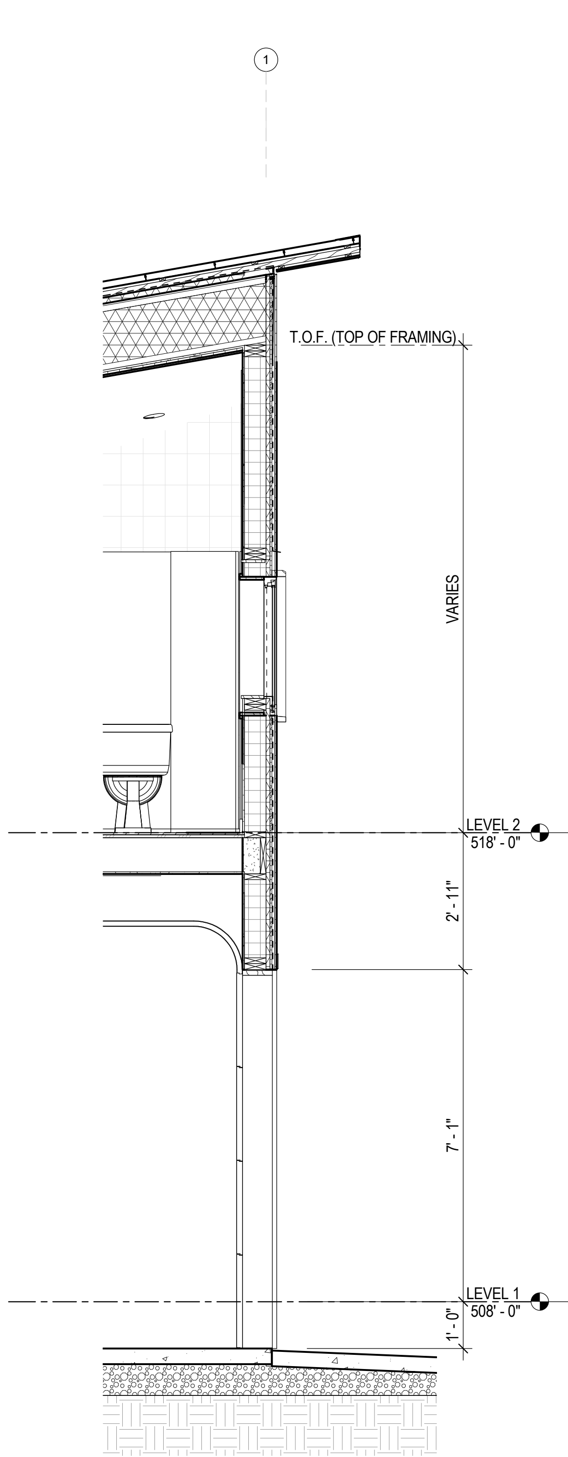
3 SECTION, GARAGE A3.21 1/2" = 1'-0"
