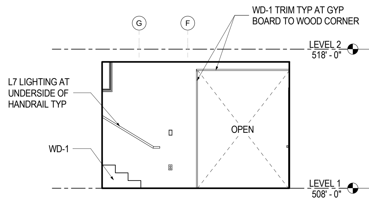
8 NORTH HALLWAY 16 - SOUTH A7.01 1/4" = 1'-0"
