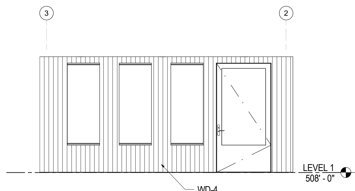
7 ENTRY HALL 01 - WEST A7.01 1/4" = 1'-0"
