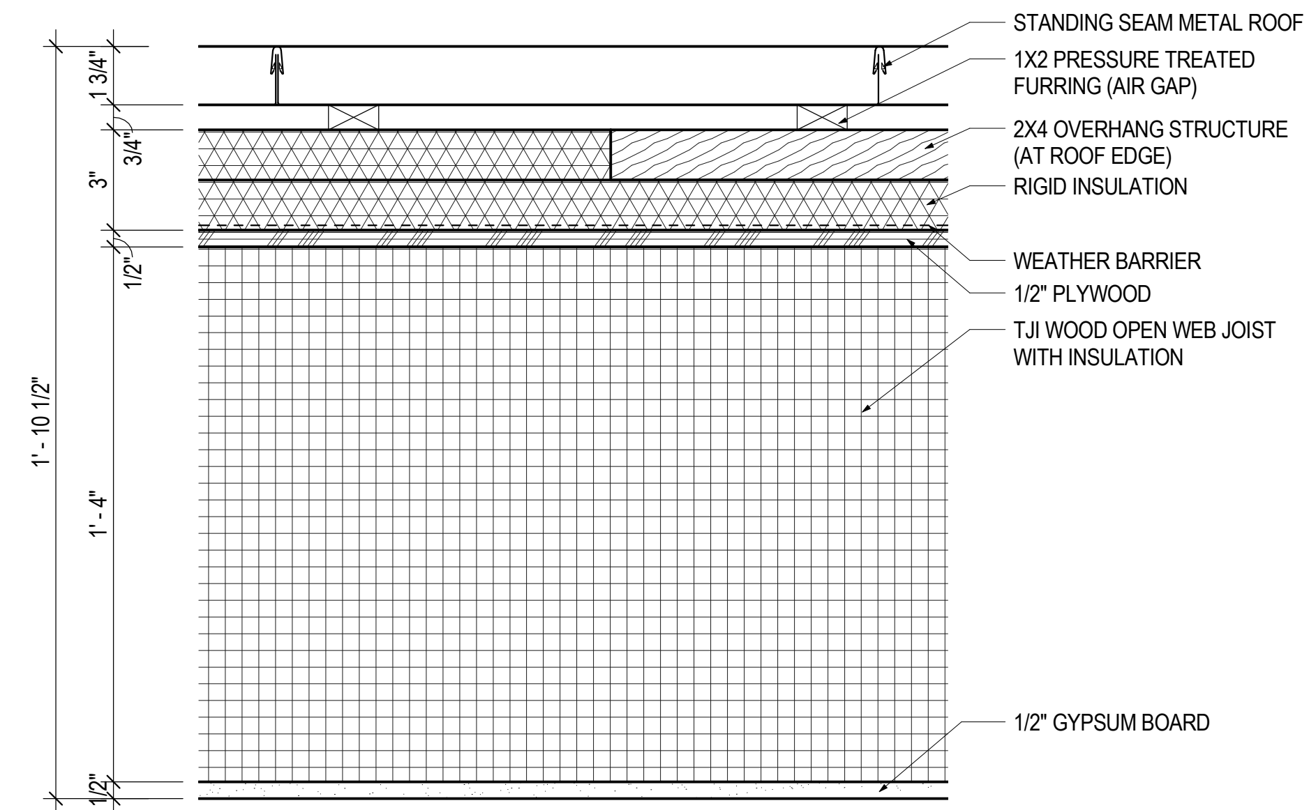
R-1 ROOF ASSEMBLY, TYPICAL 3" = 1'-0"
