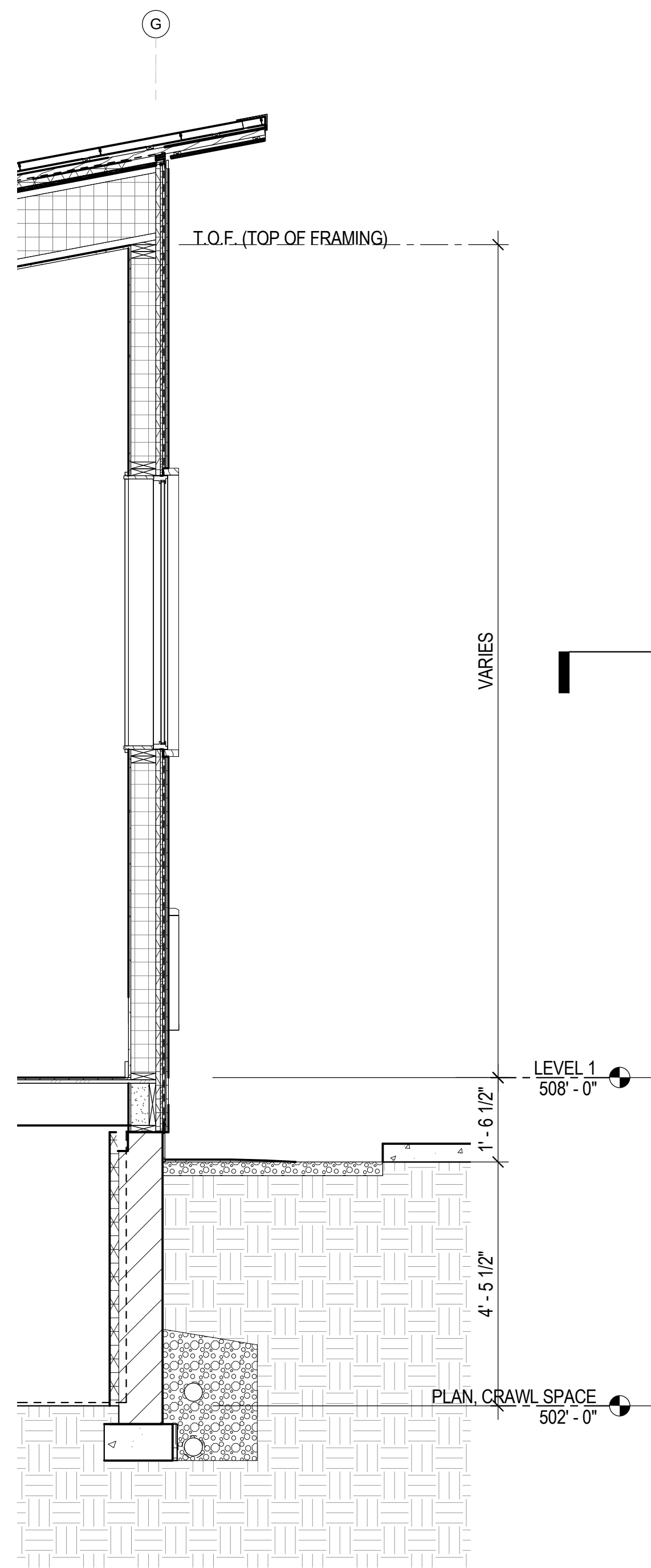
4 SECTION, TYPICAL A3.20 1/2" = 1'-0"
