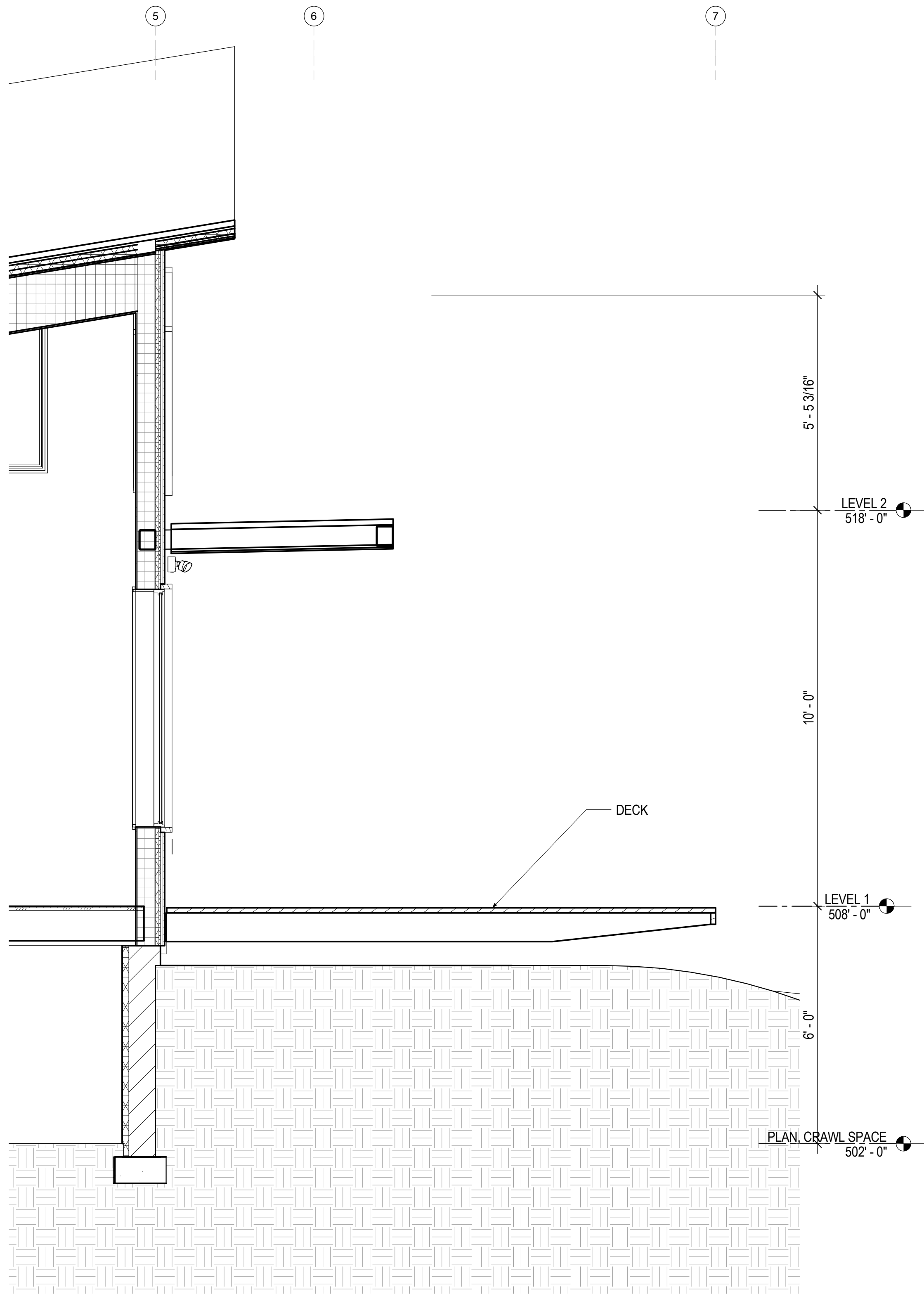
2 SECTION, DECK A5.20 1/2" = 1'-0"
