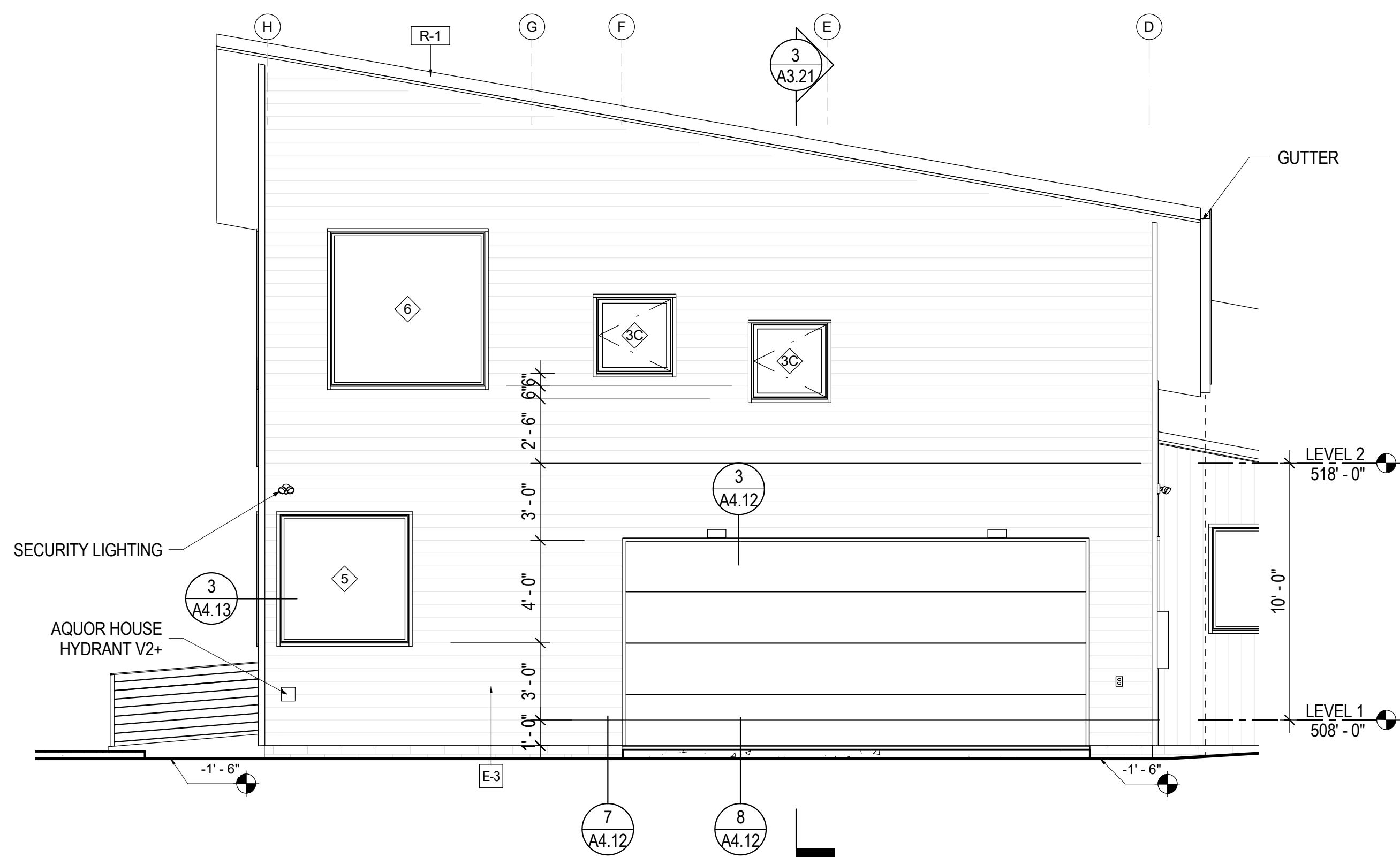
2 NORTH ELEVATION, GARAGE FACADE A3.03 1/4" = 1'-0"
