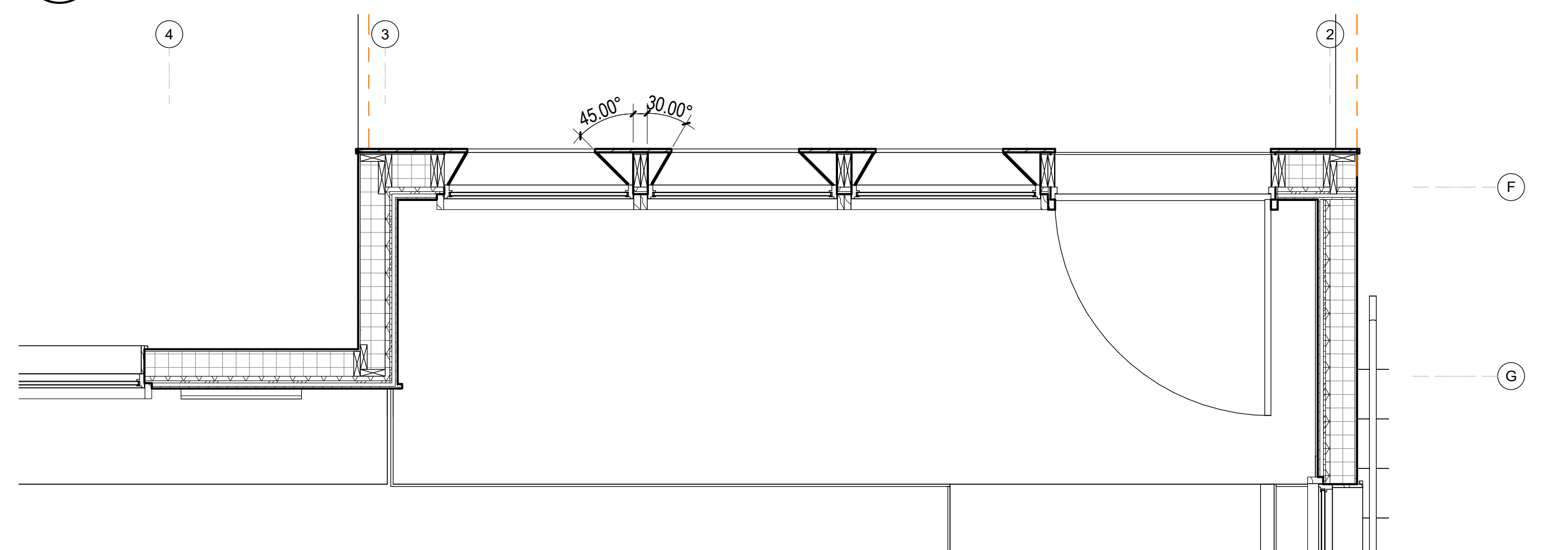
2 PLAN, ENLARGED, ENTRY HALL, EAST A3.20 1/2" = 1'-0"
