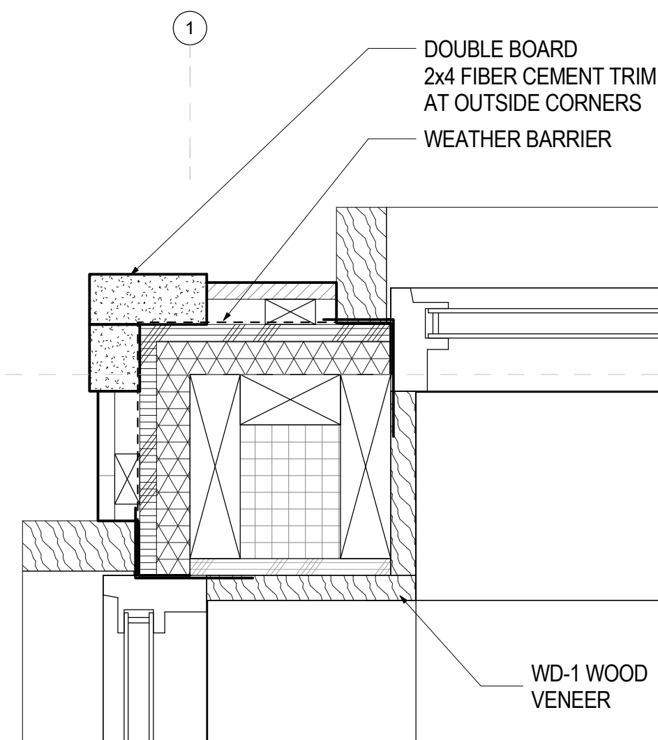
3 JAMB, CORNER WINDOW, OFFICE A4.13 3" = 1'-0"
