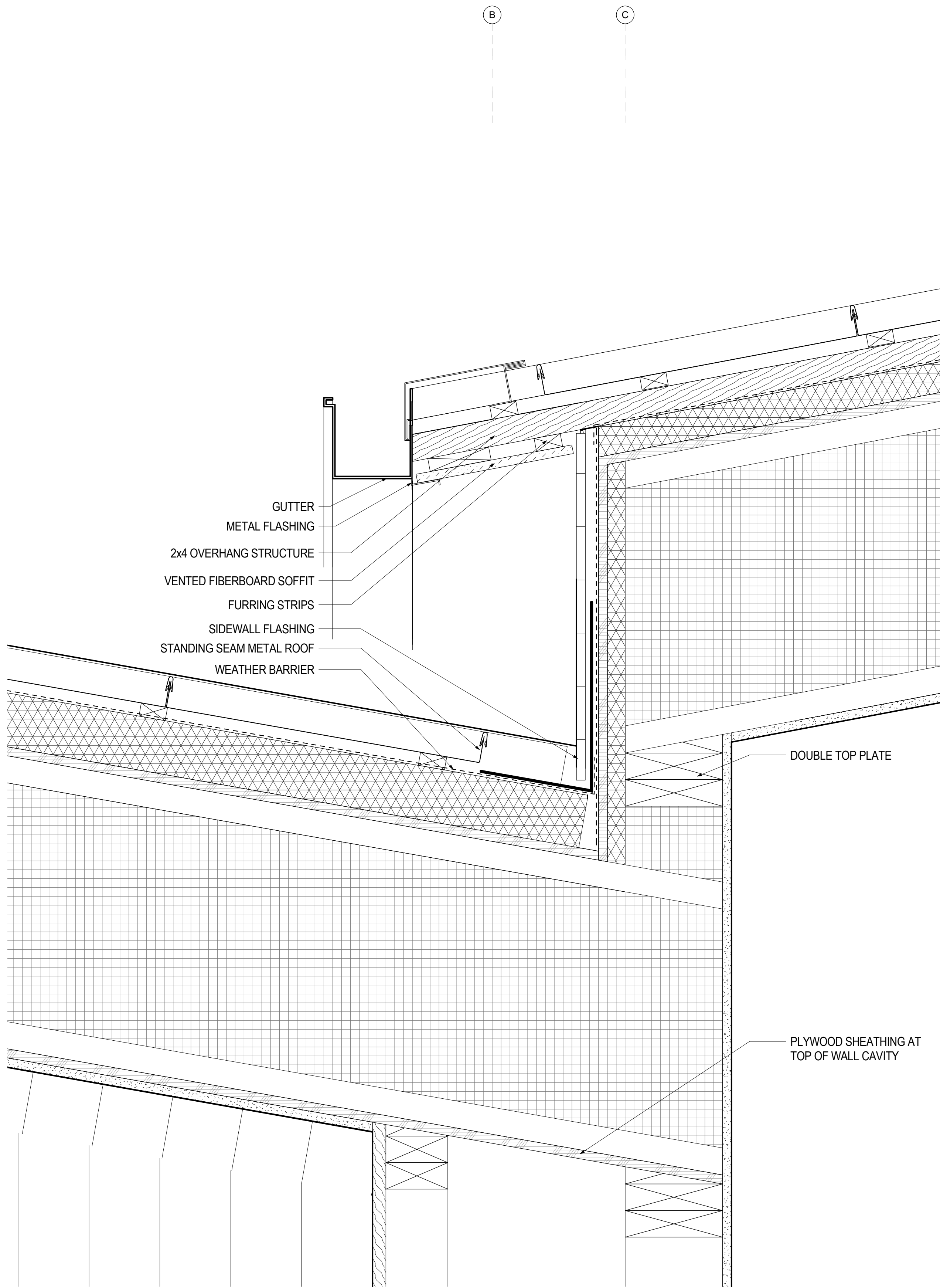
6 SECTION, ROOF INTERSECTION A4.12 3" = 1'-0"
