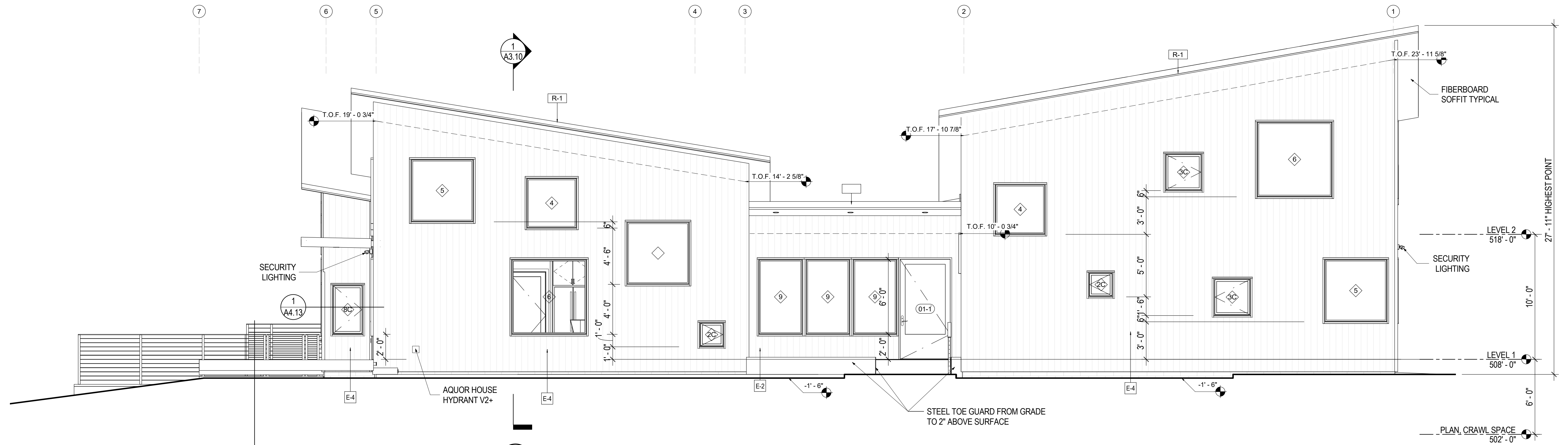
EAST ELEVATION 1 A3.10 1/4" = 1'-0"
