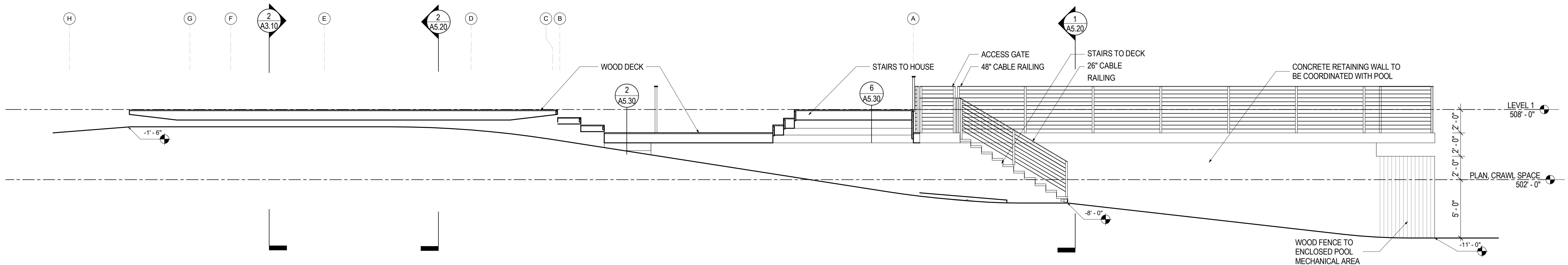
4 SOUTH SECTION, DECK A5.10 1/4" = 1'-0"
