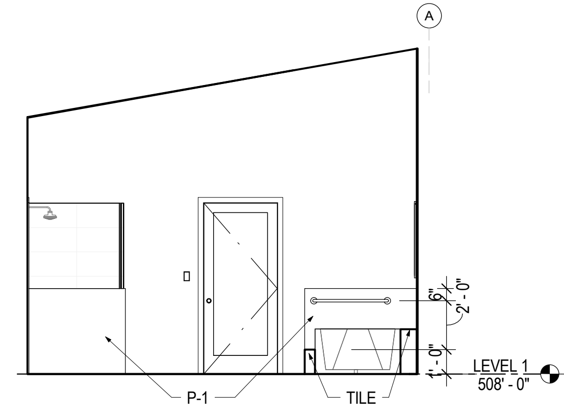
8 A7.02 MASTER BATHROOM 07 - SOUTH 1/4" = 1'-0"
