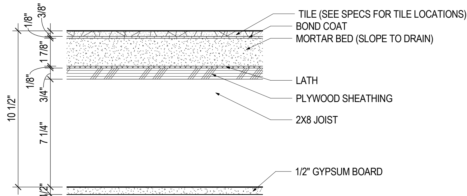
F-3 FLOOR ASSEMBLY, TILE AT SHOWER 3" = 1'-0"
