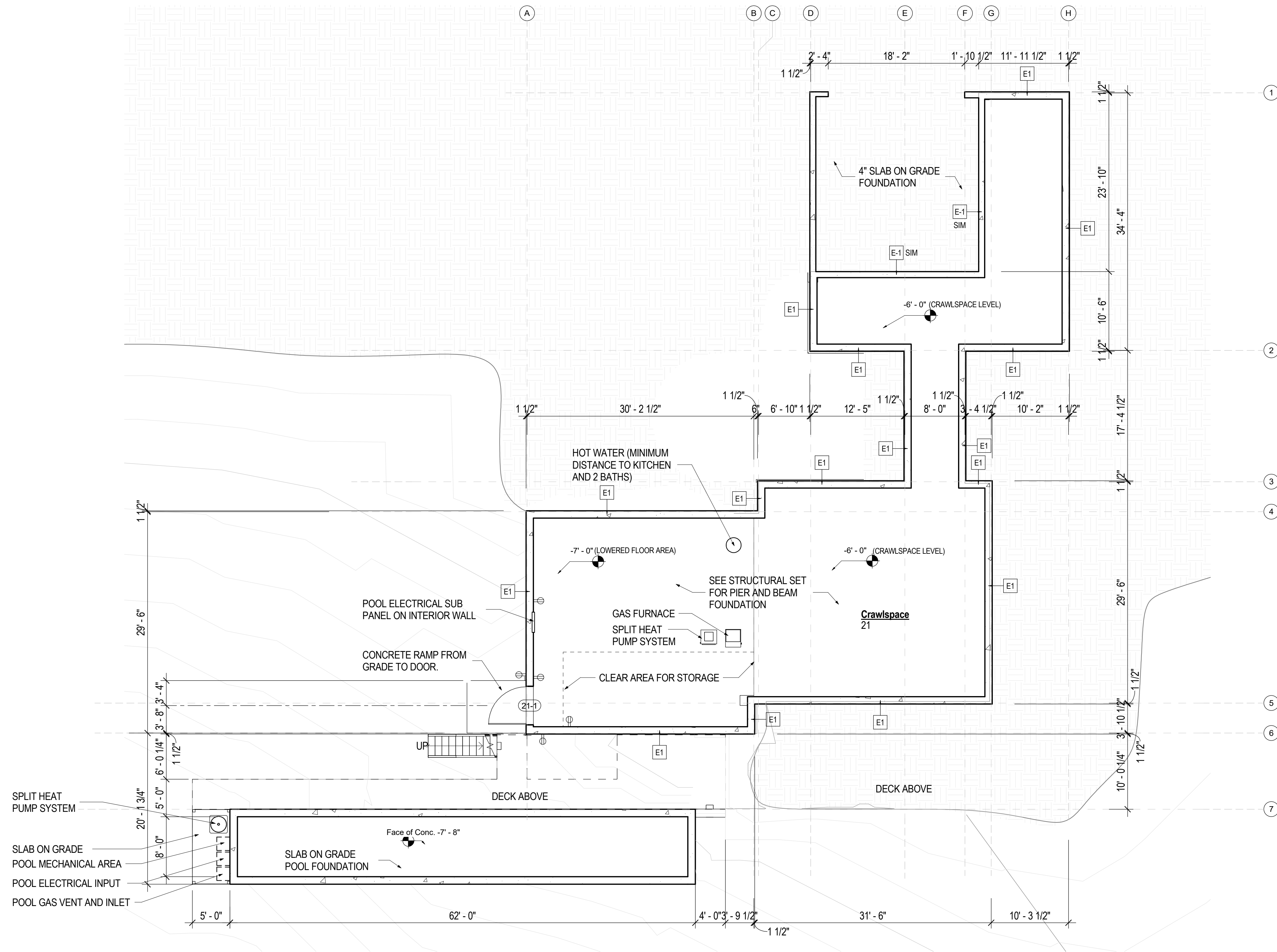
1 PLAN, CRAWL SPACE A2.00 1/8" = 1'-0"
