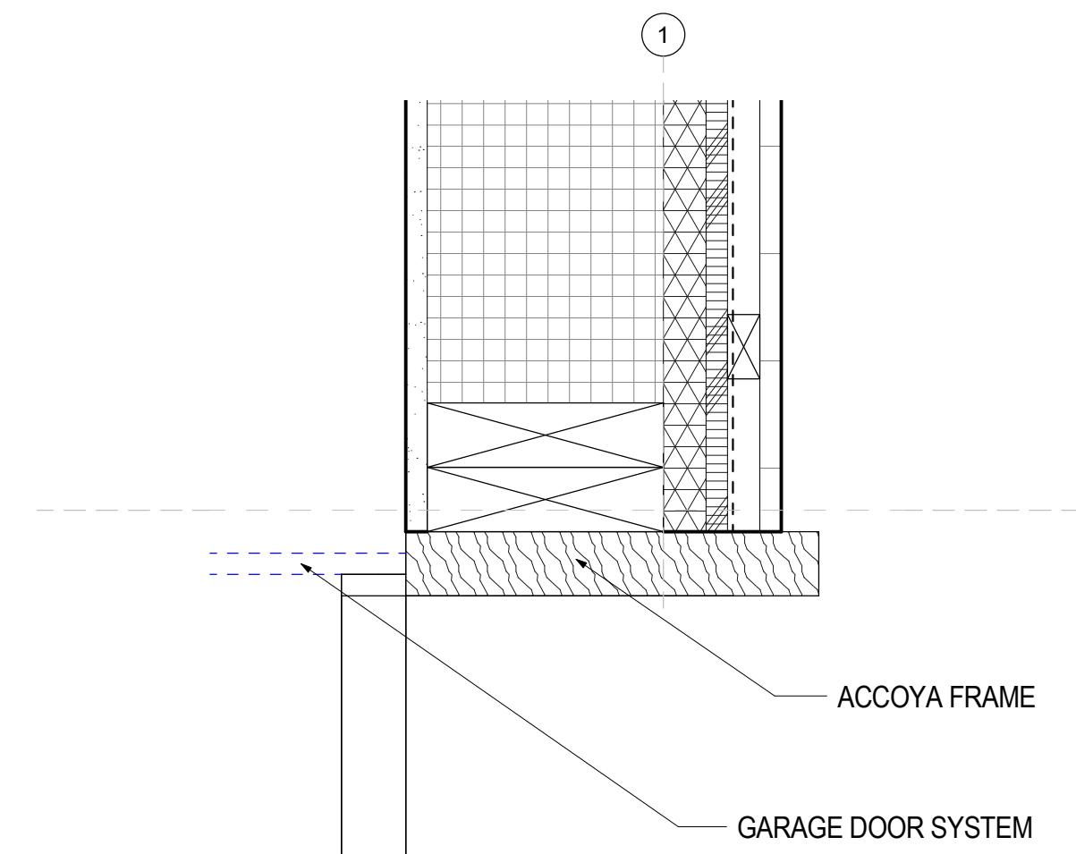
2 JAMB, GARAGE DOOR A4.12 3" = 1'-0"
