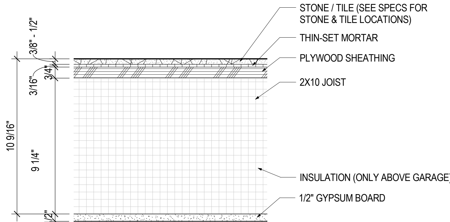
F-2 FLOOR ASSEMBLY, TILE THINSET 3" = 1'-0"
