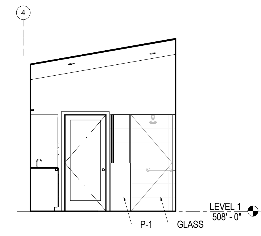
7 A7.02 MASTER BATHROOM 07 - EAST 1/4" = 1'-0"
