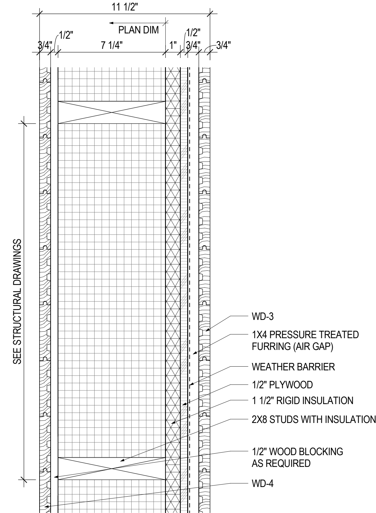
E-2 EXTERIOR WALL, WOOD CONNECTOR 3" = 1'-0"
