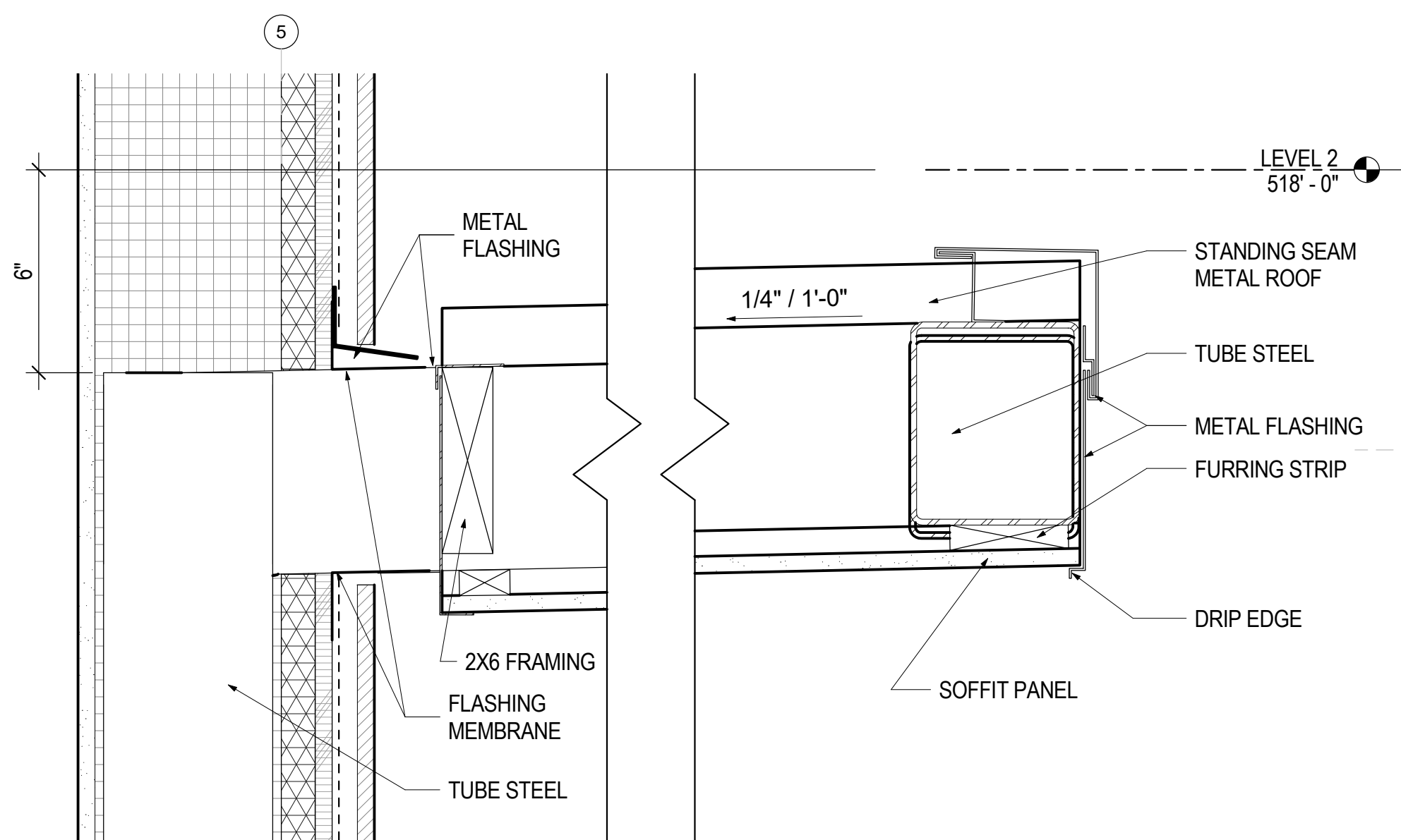
5 SECTION, PORCH OVERHANG A4.13 3" = 1'-0"
