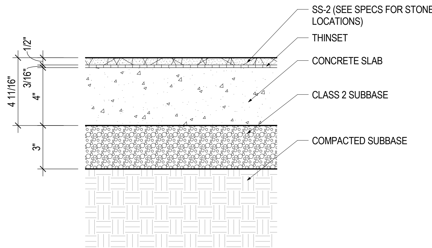
F-6 FLOOR ASSEMBLY, EXTERIOR STONE 3" = 1'-0"
