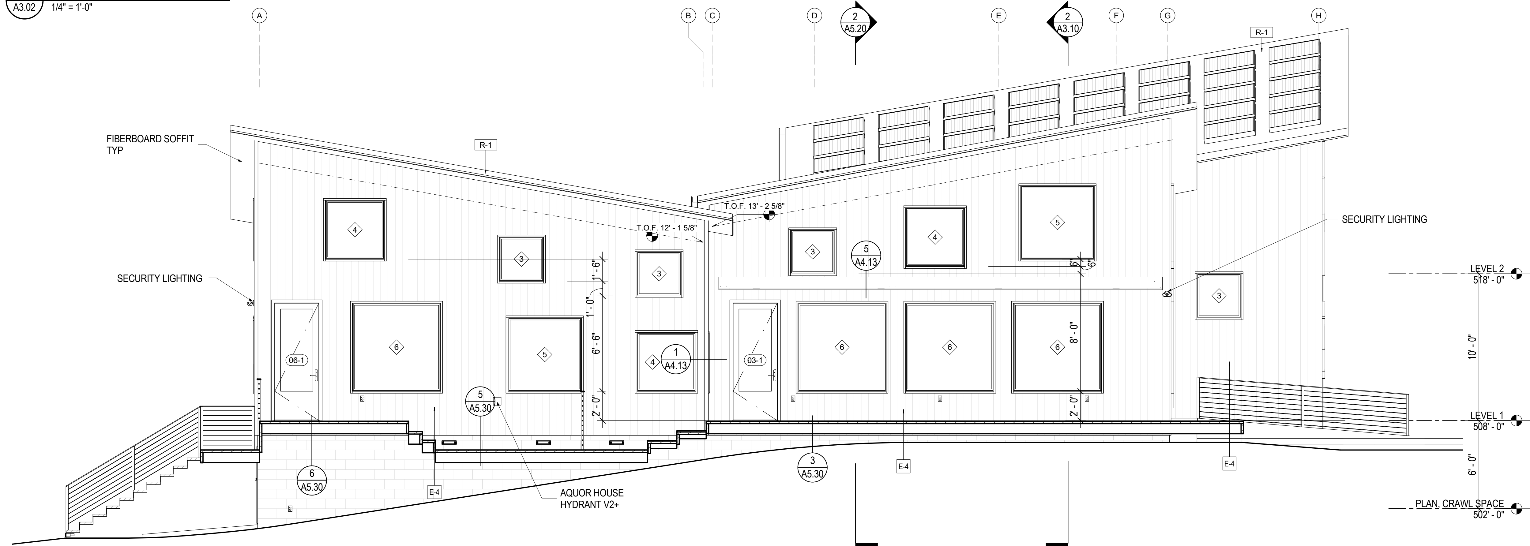
2 SOUTH ELEVATION A3.02 1/4" = 1'-0"
