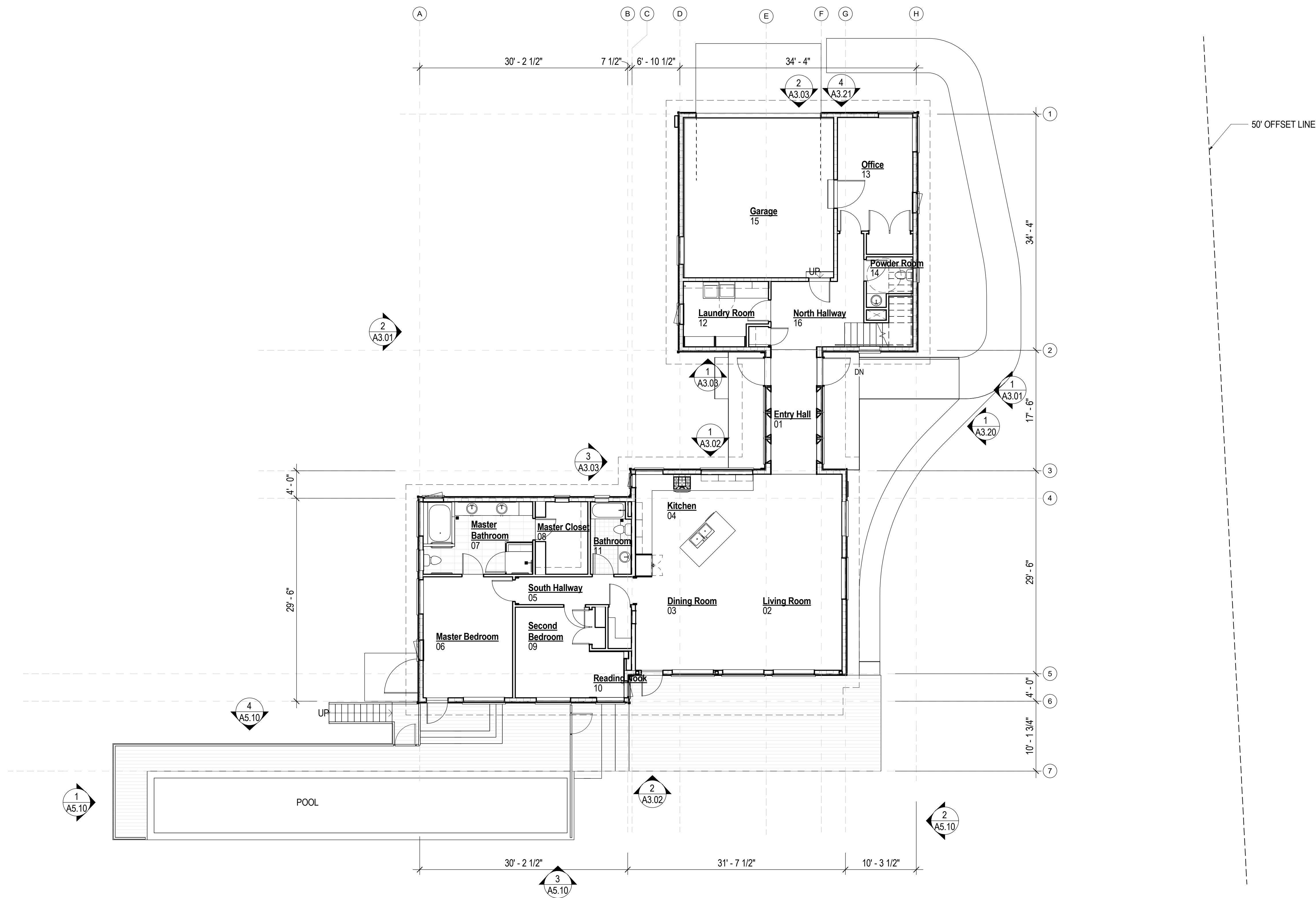
1 PLAN, LEVEL 1 A2.01 1/8" = 1'-0"
