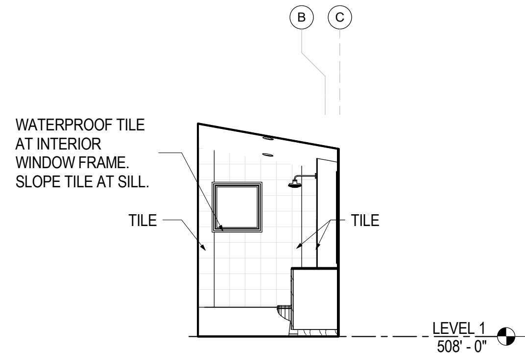
3 A7.02 BATHROOM 11 - NORTH 1/4" = 1'-0"
