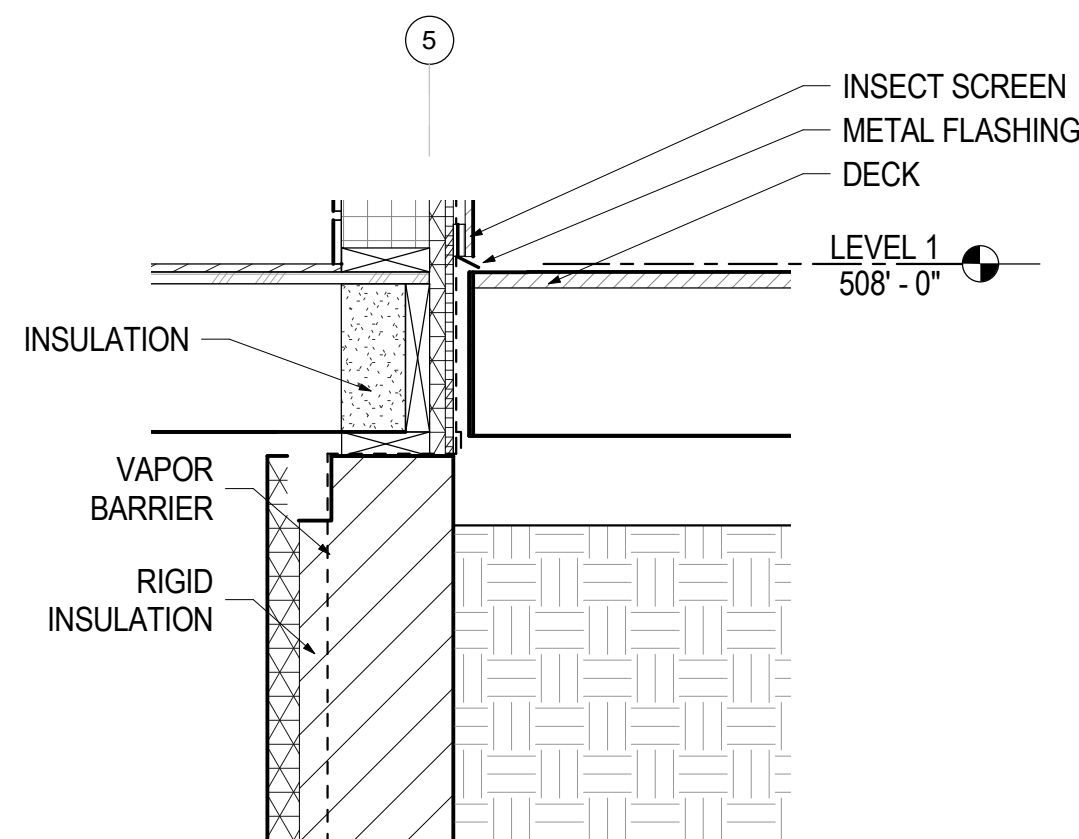
3 BASE, UPPER DECK 1" = 1'-0"
