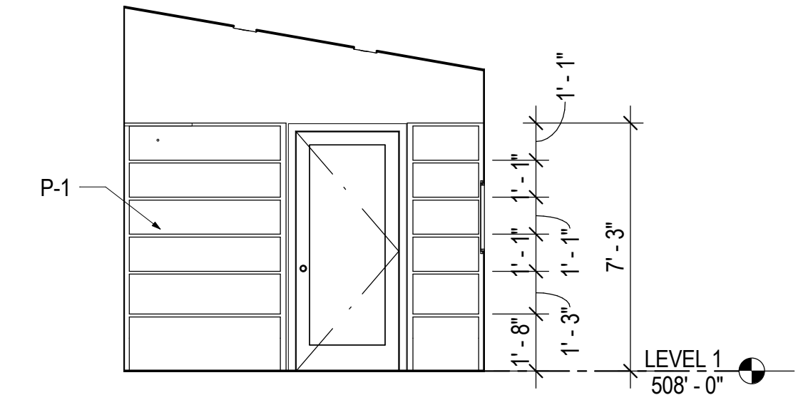
1 A7.02 MASTER CLOSET 08 - WEST 1/4" = 1'-0"
