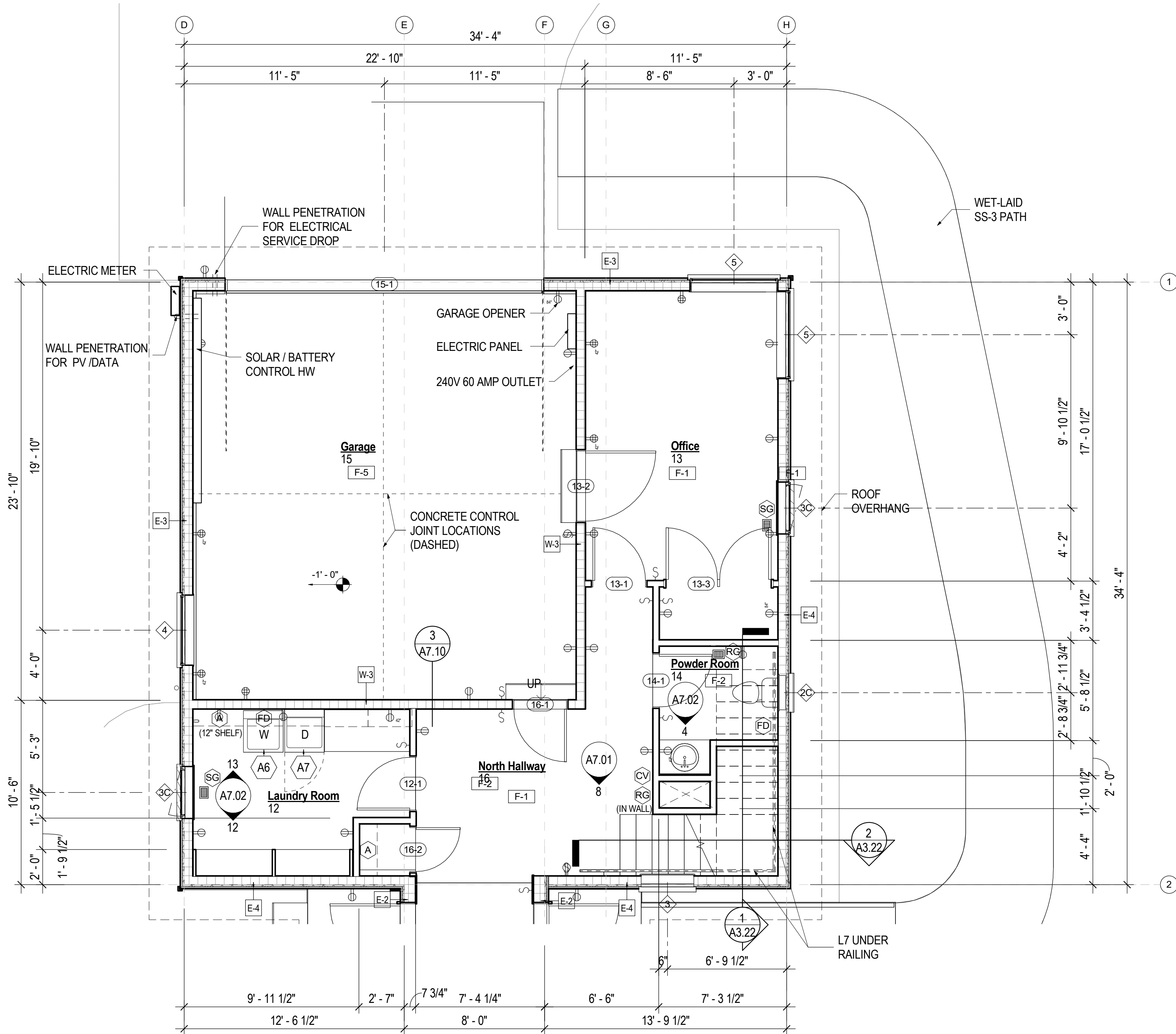
1 ENLARGED PLAN, LEVEL 1 NORTH A2.01B 1/4" = 1'-0"
