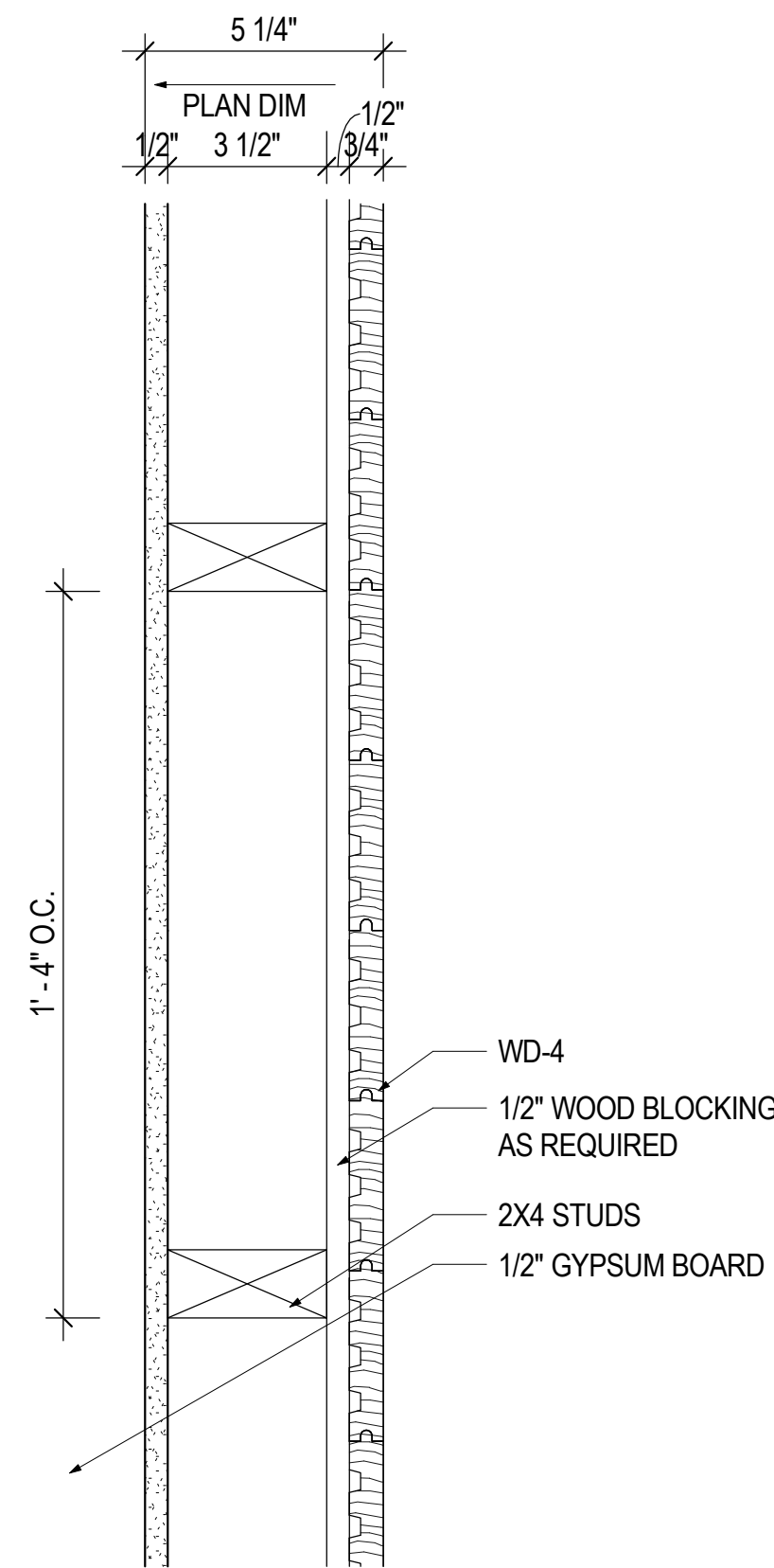
W-4 INTERIOR WALL, 2X4 WOOD VENEER 3" = 1'-0"
