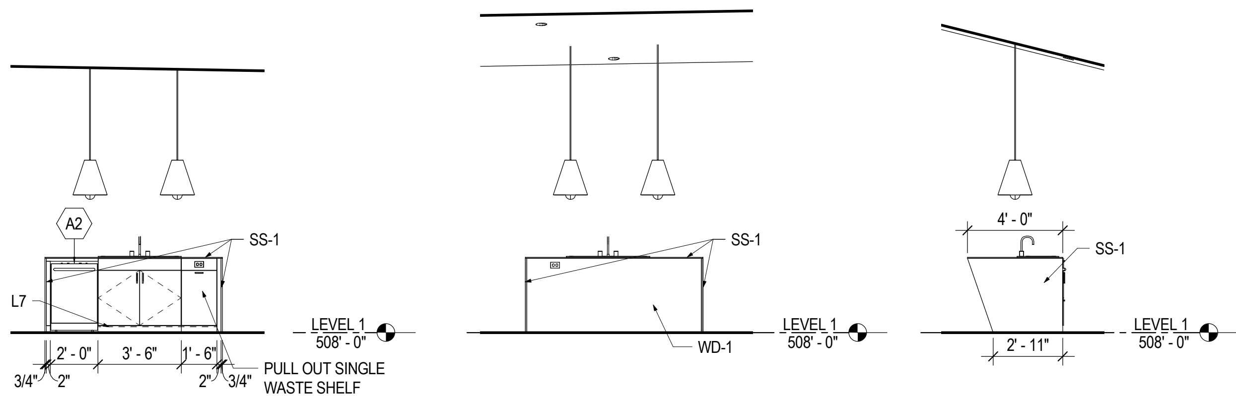
5 KITCHEN 04 - ISLAND EAST A7.01 1/4" = 1'-0"
