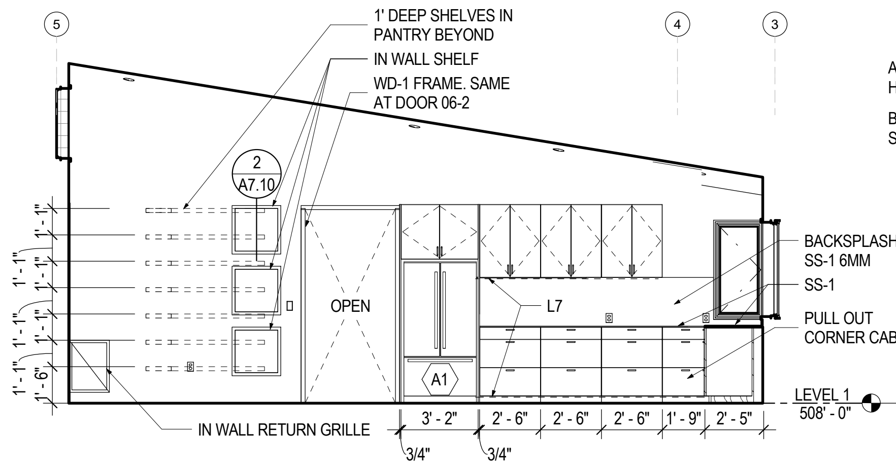
2 KITCHEN 04 - WEST A7.01 1/4" = 1'-0"
