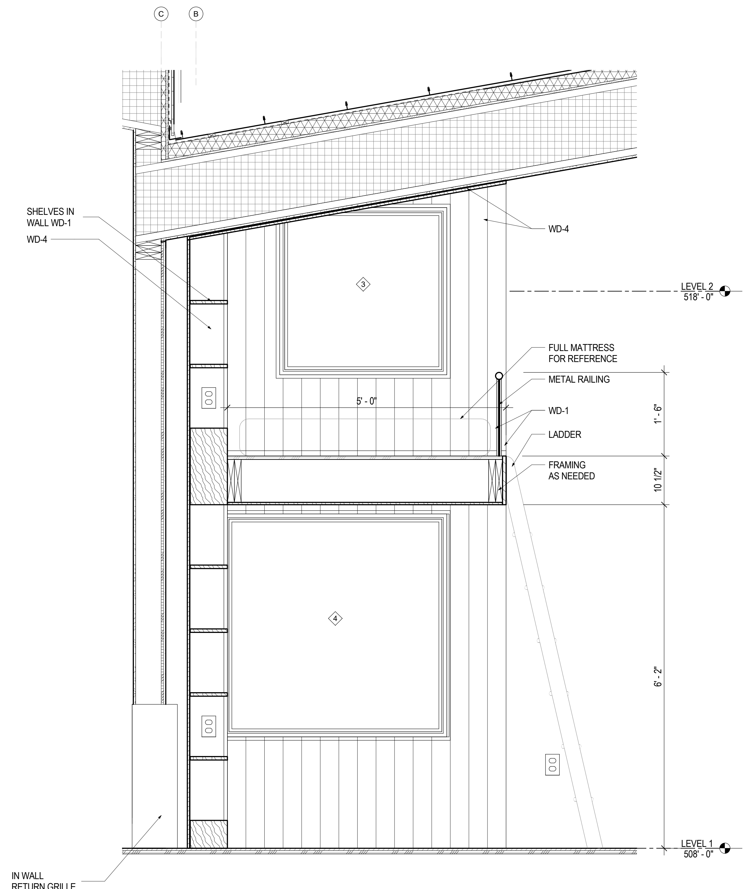
1 A7.10 SECTION, READING NOOK 1" = 1'-0"
