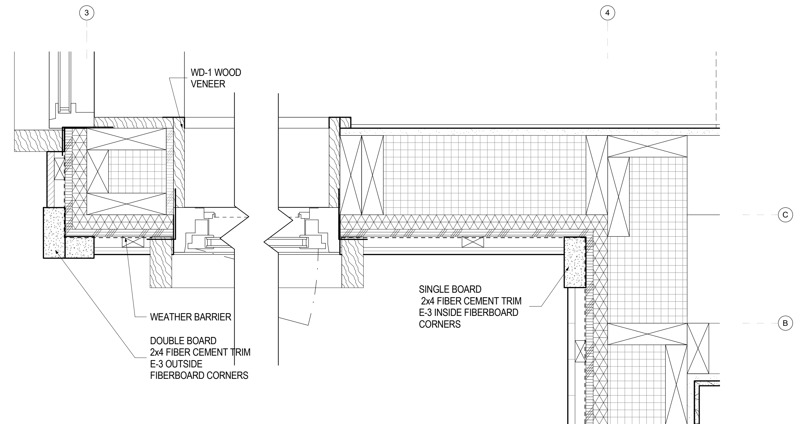
2 JAMB, CORNER WINDOW, KITCHEN A4.13 3" = 1'-0"
