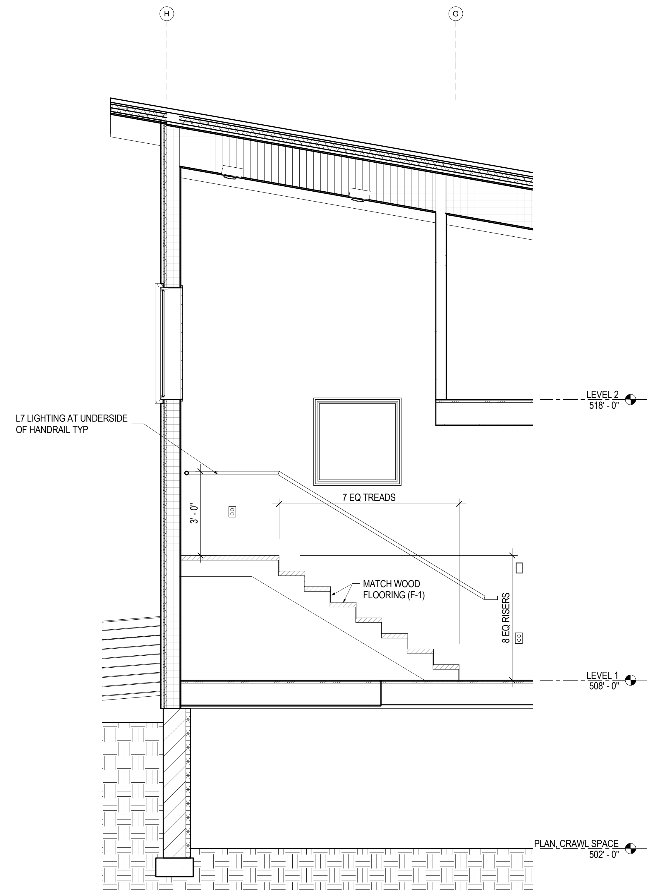
2 A3.22 SECTION, STAIRS SOUTH 1/2" = 1'-0"
