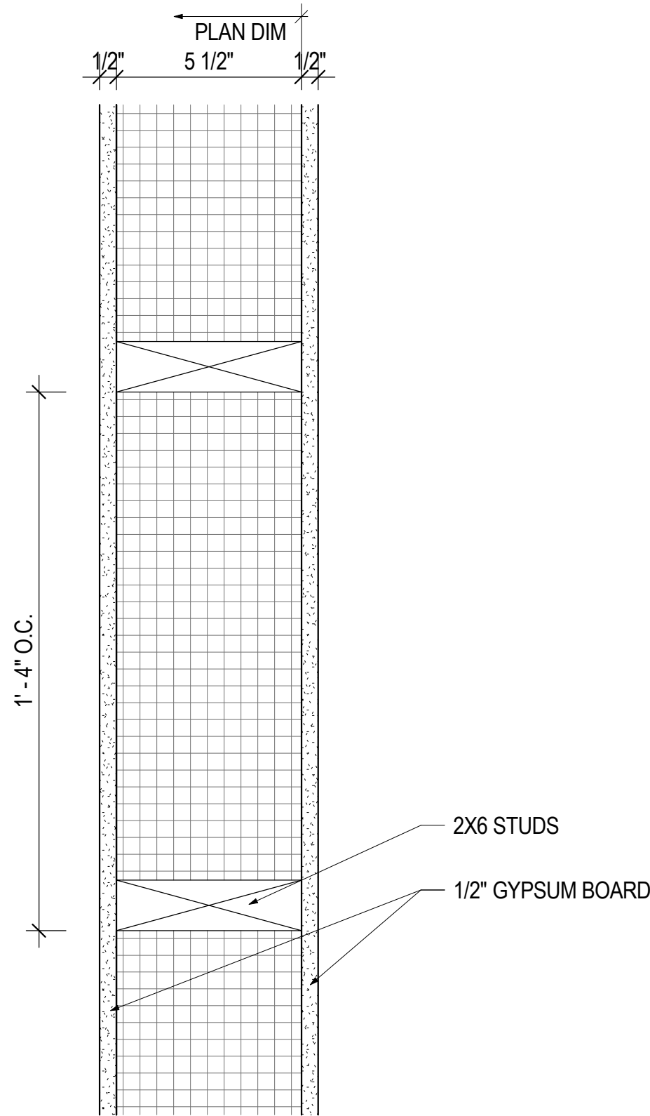
W-3 INTERIOR WALL, INSULATED 3" = 1'-0"
