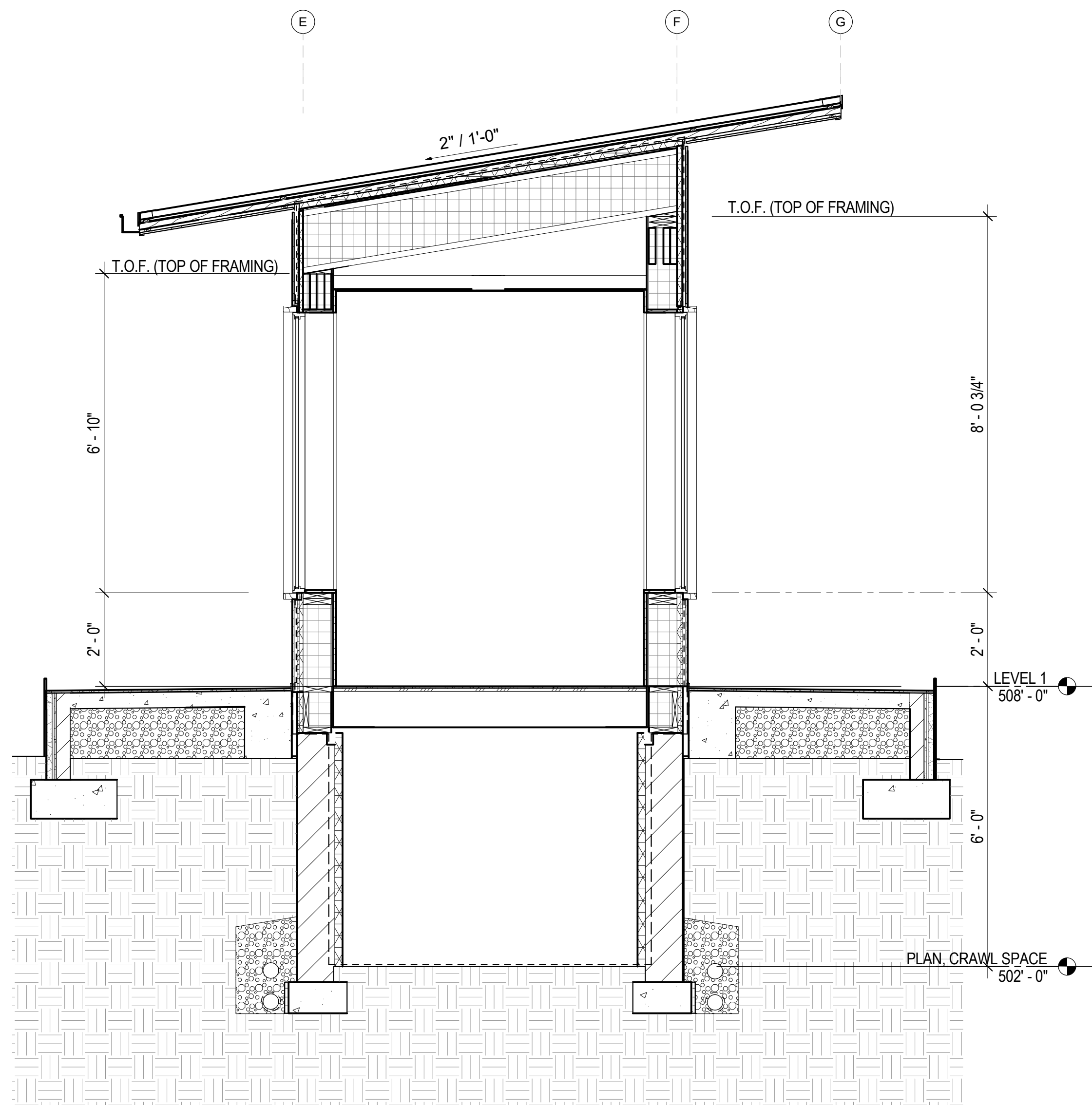
3 SECTION, ENTRY HALL A3.20 1/2" = 1'-0"
