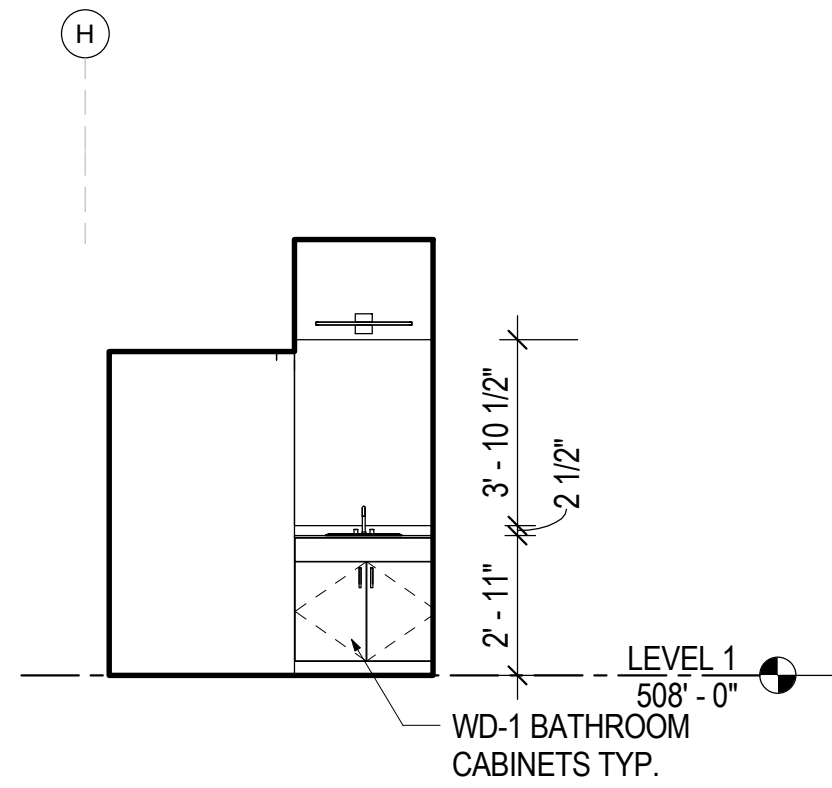
4 A7.02 POWDER ROOM 14 - SOUTH 1/4" = 1'-0"
