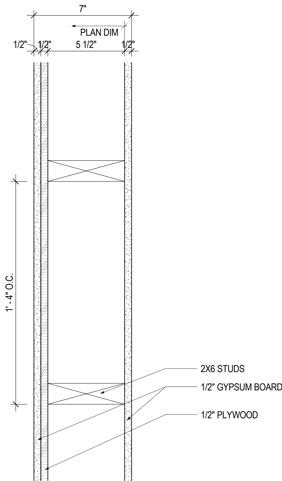
W-2 INTERIOR WALL, 2X6 3" = 1'-0"
