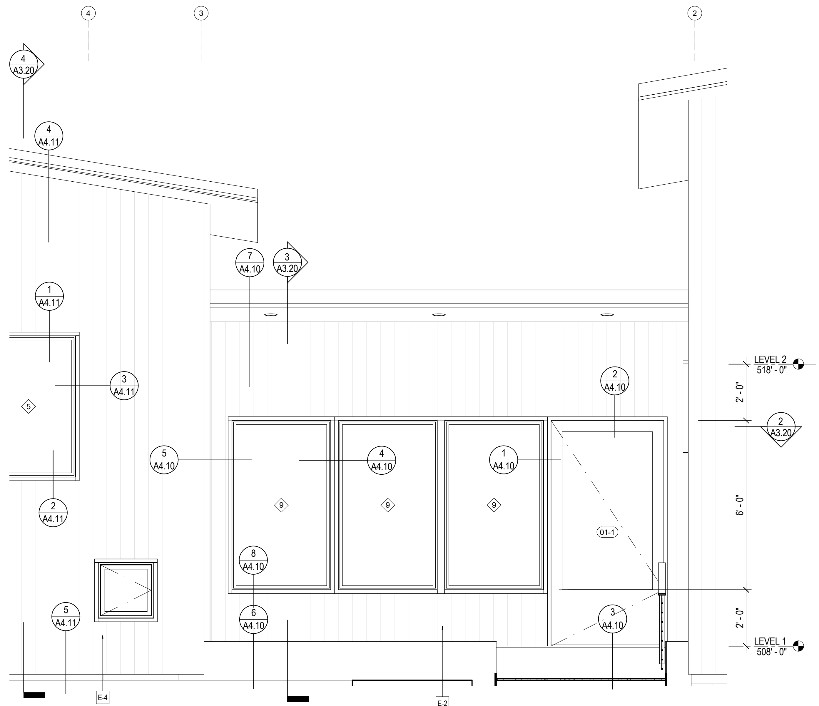
1 PARTIAL ELEVATION, ENTRY HALL, EAST A3.20 1/2" = 1'-0"
