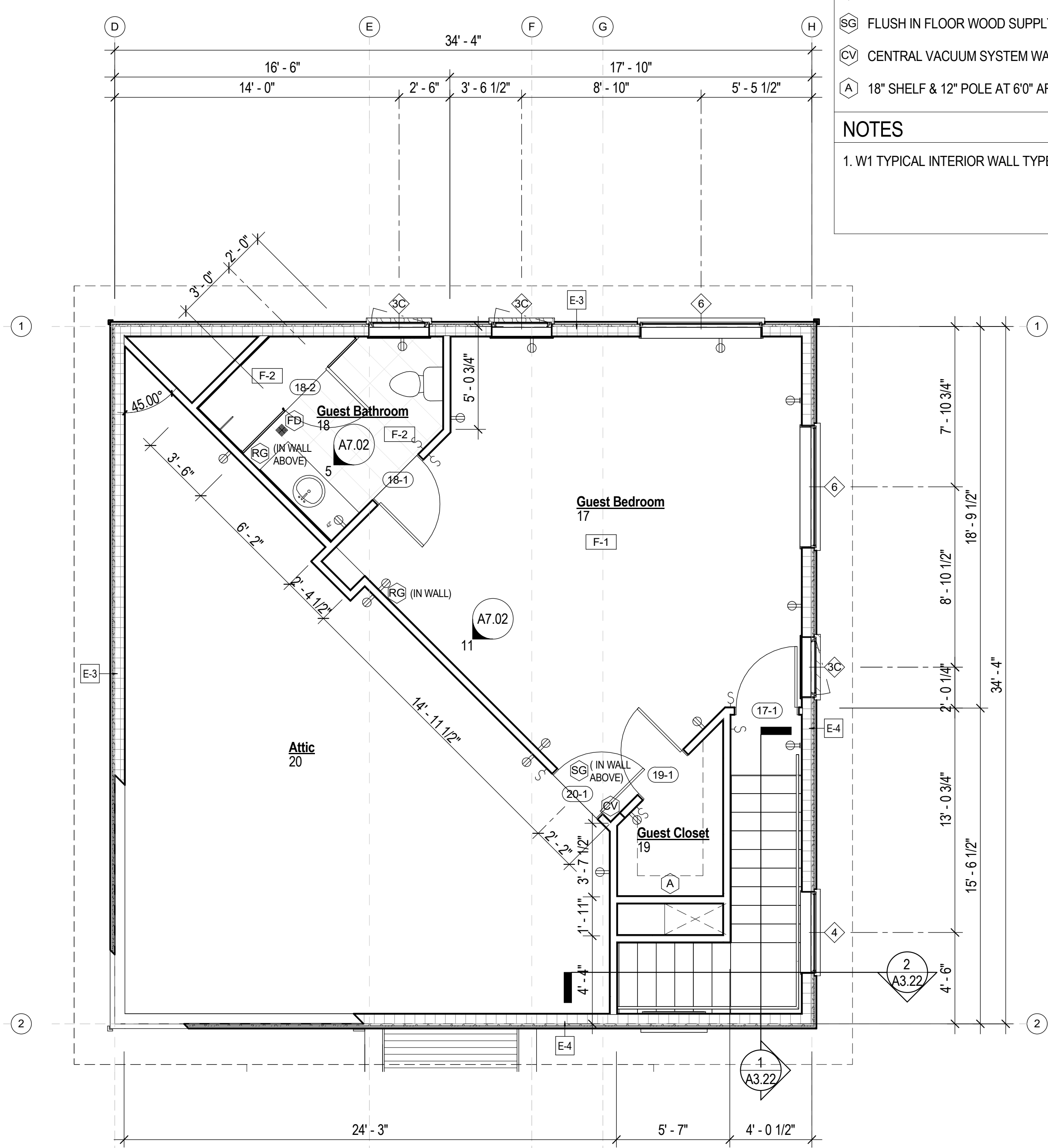
2 ENLARGED PLAN, LEVEL 2 NORTH A2.01B 1/4" = 1'-0"
