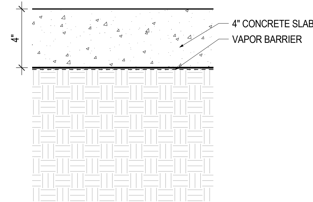
F-5 FLOOR ASSEMBLY, GARAGE 3" = 1'-0"
