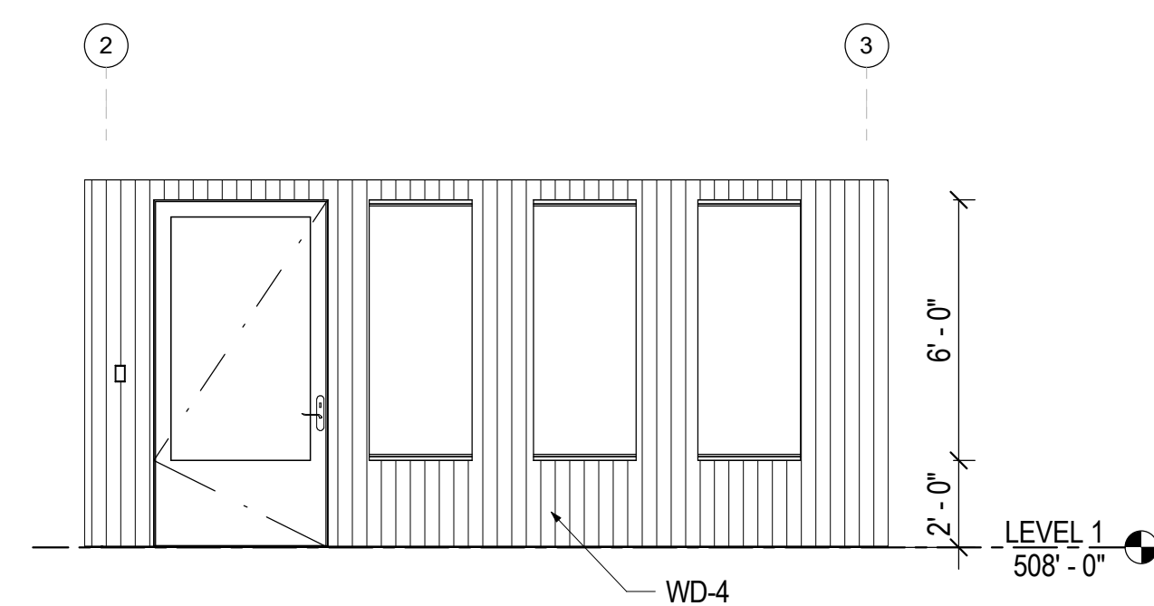
6 ENTRY HALL 01 - EAST A7.01 1/4" = 1'-0"
