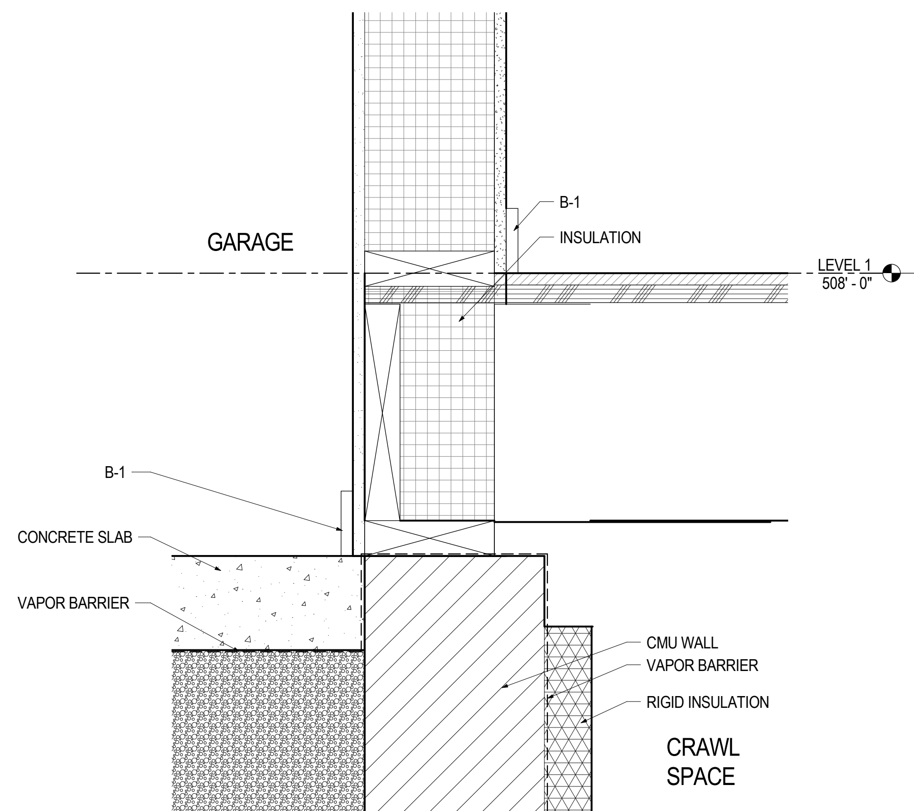
3 A7.10 BASE, GARAGE, INTERIOR 3" = 1'-0"
