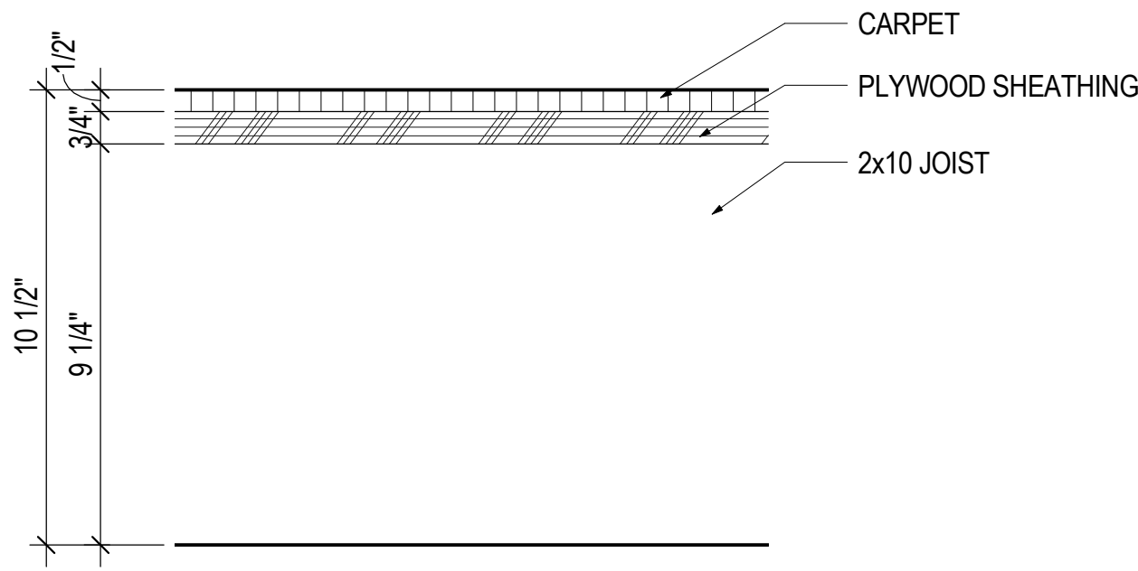
F-4 FLOOR ASSEMBLY, CARPET 3" = 1'-0"
