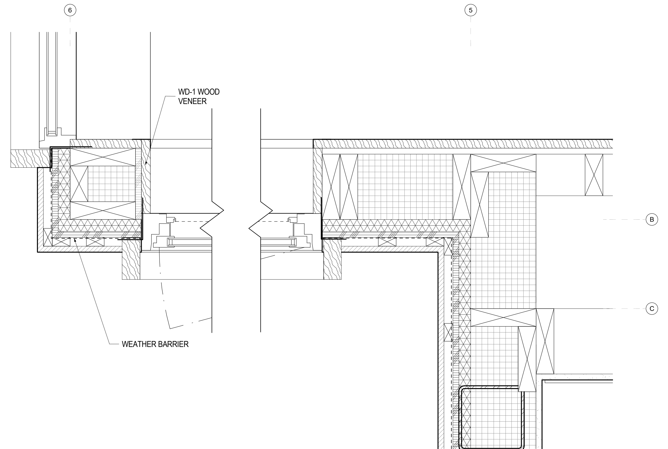
1 JAMB, CORNER WINDOW, READING NOOK A4.13 3" = 1'-0"
