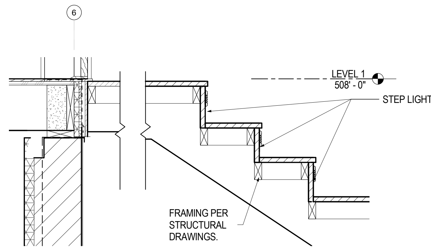
6 SECTION, MASTER BEDROOM TO DECK 1" = 1'-0"
