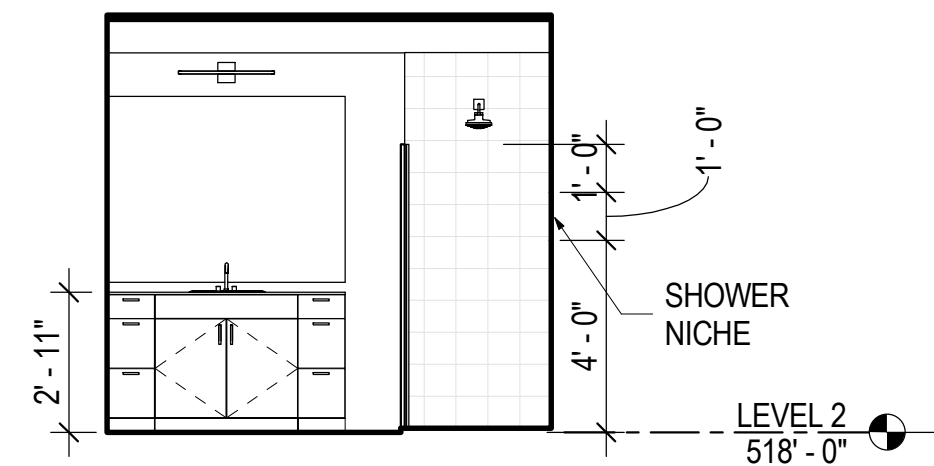
5 A7.02 GUEST BATHROOM 19 - SOUTH 1/4" = 1'-0"
