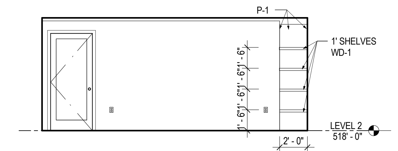
11 A7.02 GUEST BEDROOM 17 - WEST 1/4" = 1'-0"
