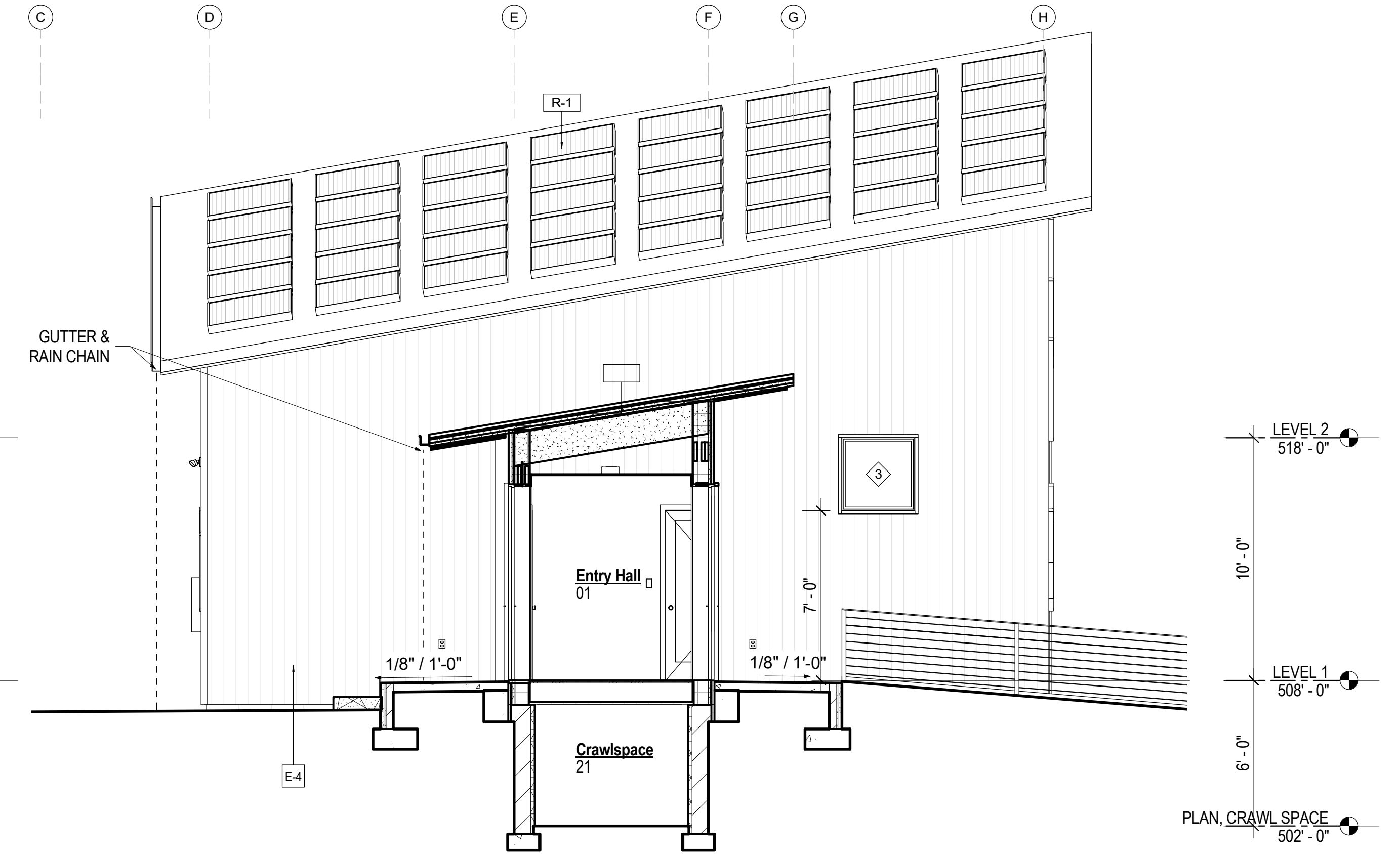
1 SOUTH ELEVATION, LAUNDRY / GUEST BED FACADE A3.03 1/4" = 1'-0"
